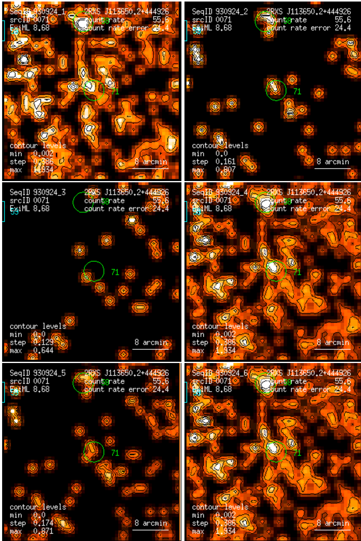
Figure 71: RASS 930924: detection 0071: band rate images, Gaussian filter: (1) PSPC channels 11 – 41, (2) 52 – 90, (3) 91 – 201, (4) 11 – 235, (5) 52 – 201, (6) 11 – 201. Broad band rates in counts/ks. Band rate contour levels in counts/ks/arcmin 2 .
