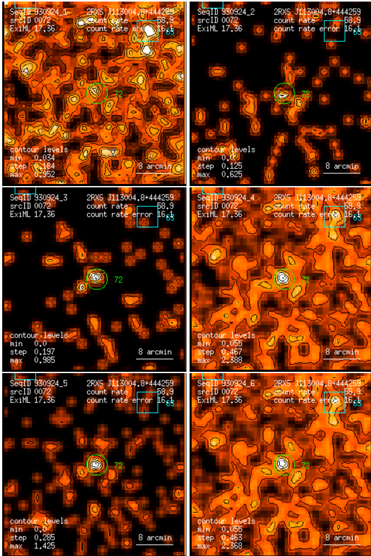
Figure 72: RASS 930924: detection 0072: band rate images, Gaussian filter: (1) PSPC channels 11 – 41, (2) 52 – 90, (3) 91 – 201, (4) 11 – 235, (5) 52 – 201, (6) 11 – 201. Broad band rates in counts/ks. Band rate contour levels in counts/ks/arcmin 2 .
