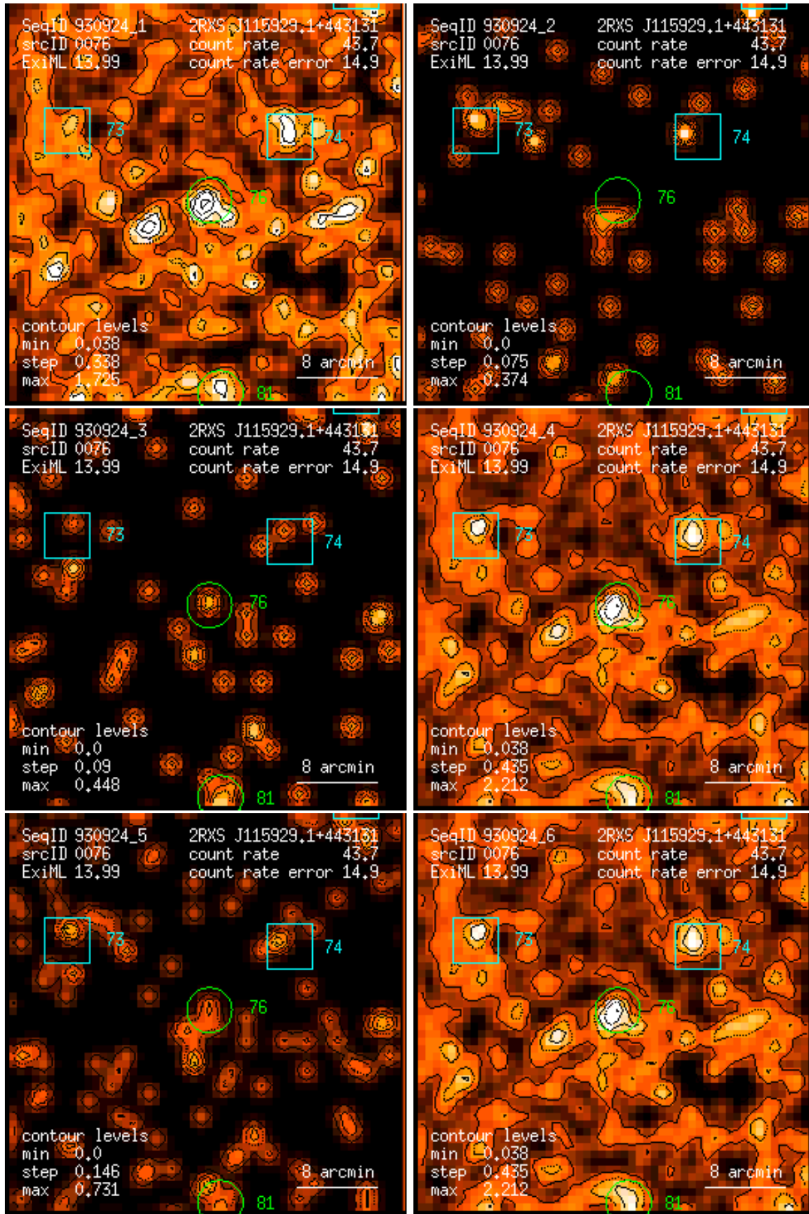
Figure 76: RASS 930924: detection 0076: band rate images, Gaussian filter: (1) PSPC channels 11 – 41, (2) 52 – 90, (3) 91 – 201, (4) 11 – 235, (5) 52 – 201, (6) 11 – 201. Broad band rates in counts/ks. Band rate contour levels in counts/ks/arcmin 2 .
