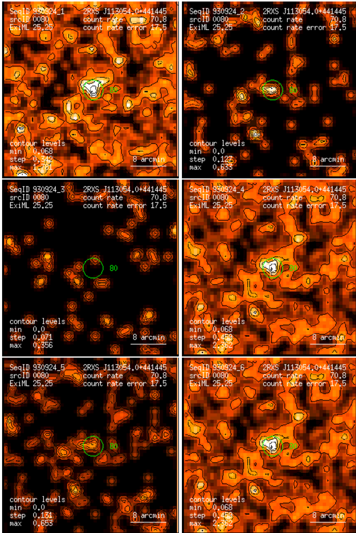
Figure 80: RASS 930924: detection 0080: band rate images, Gaussian filter: (1) PSPC channels 11 – 41, (2) 52 – 90, (3) 91 – 201, (4) 11 – 235, (5) 52 – 201, (6) 11 – 201. Broad band rates in counts/ks. Band rate contour levels in counts/ks/arcmin 2 .
