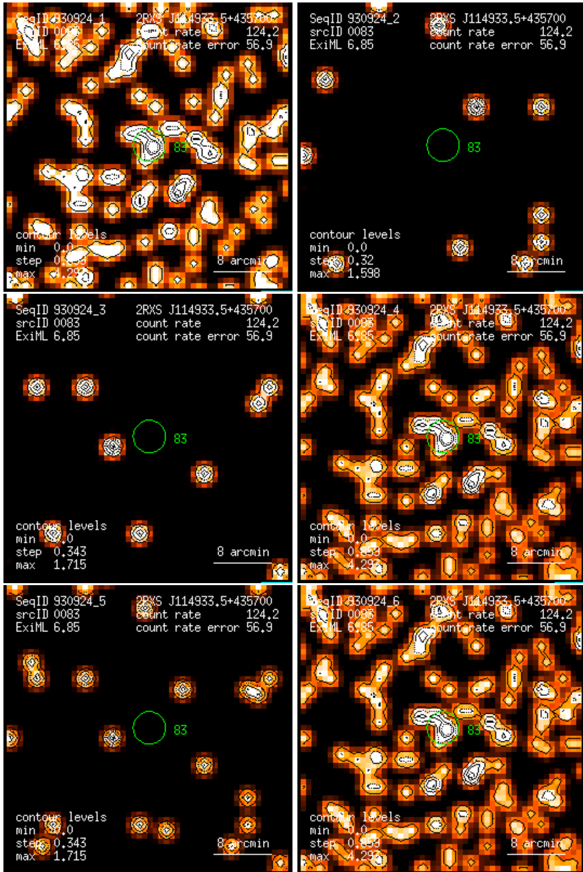
Figure 83: RASS 930924: detection 0083: band rate images, Gaussian filter: (1) PSPC channels 11 – 41, (2) 52 – 90, (3) 91 – 201, (4) 11 – 235, (5) 52 – 201, (6) 11 – 201. Broad band rates in counts/ks. Band rate contour levels in counts/ks/arcmin 2 .
