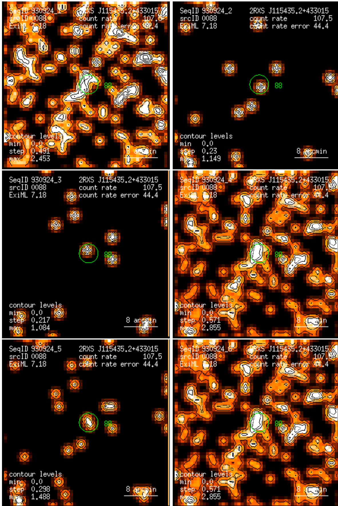
Figure 88: RASS 930924: detection 0088: band rate images, Gaussian filter: (1) PSPC channels 11 – 41, (2) 52 – 90, (3) 91 – 201, (4) 11 – 235, (5) 52 – 201, (6) 11 – 201. Broad band rates in counts/ks. Band rate contour levels in counts/ks/arcmin 2 .
