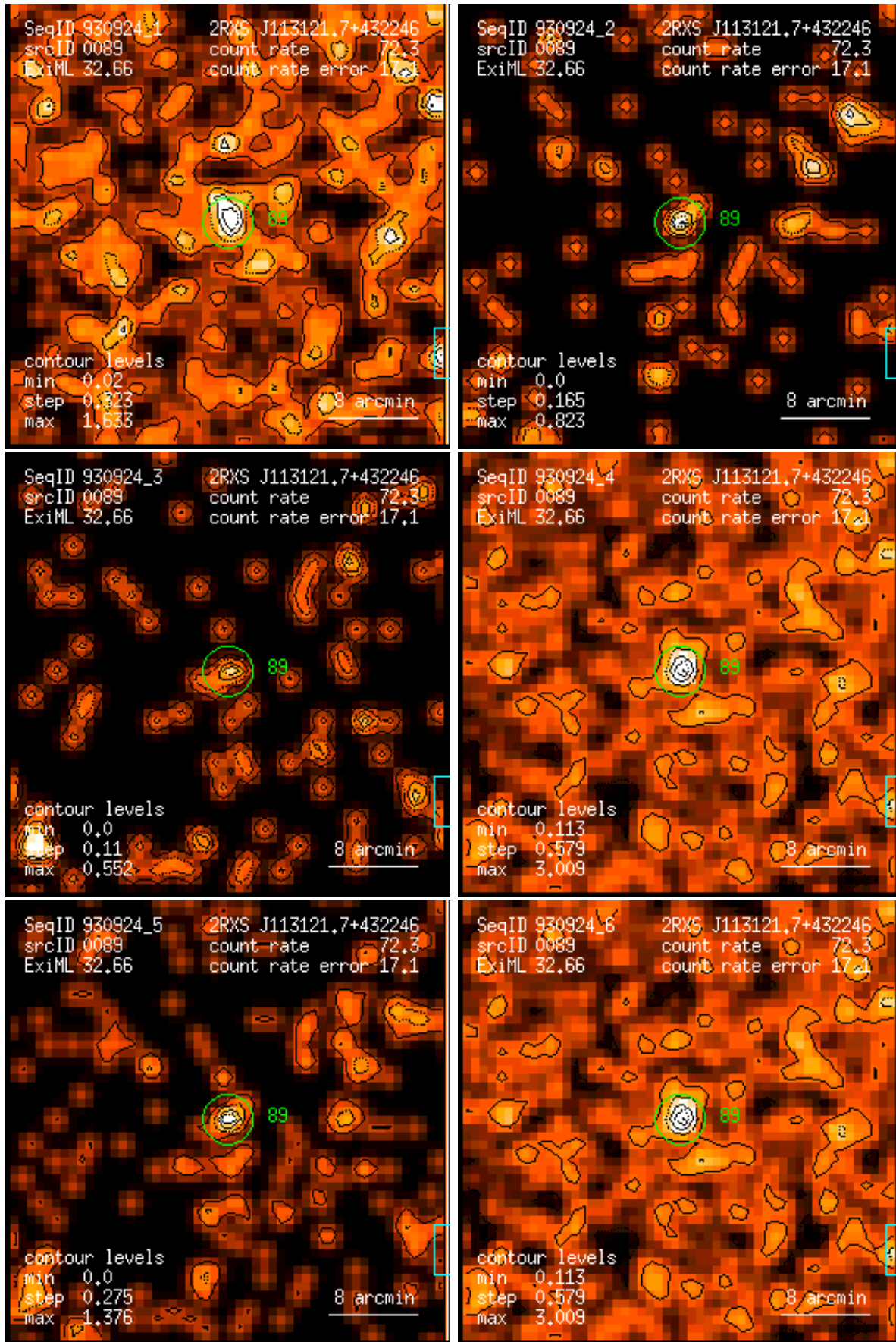
Figure 89: RASS 930924: detection 0089: band rate images, Gaussian filter: (1) PSPC channels 11 – 41, (2) 52 – 90, (3) 91 – 201, (4) 11 – 235, (5) 52 – 201, (6) 11 – 201. Broad band rates in counts/ks. Band rate contour levels in counts/ks/arcmin 2 .
