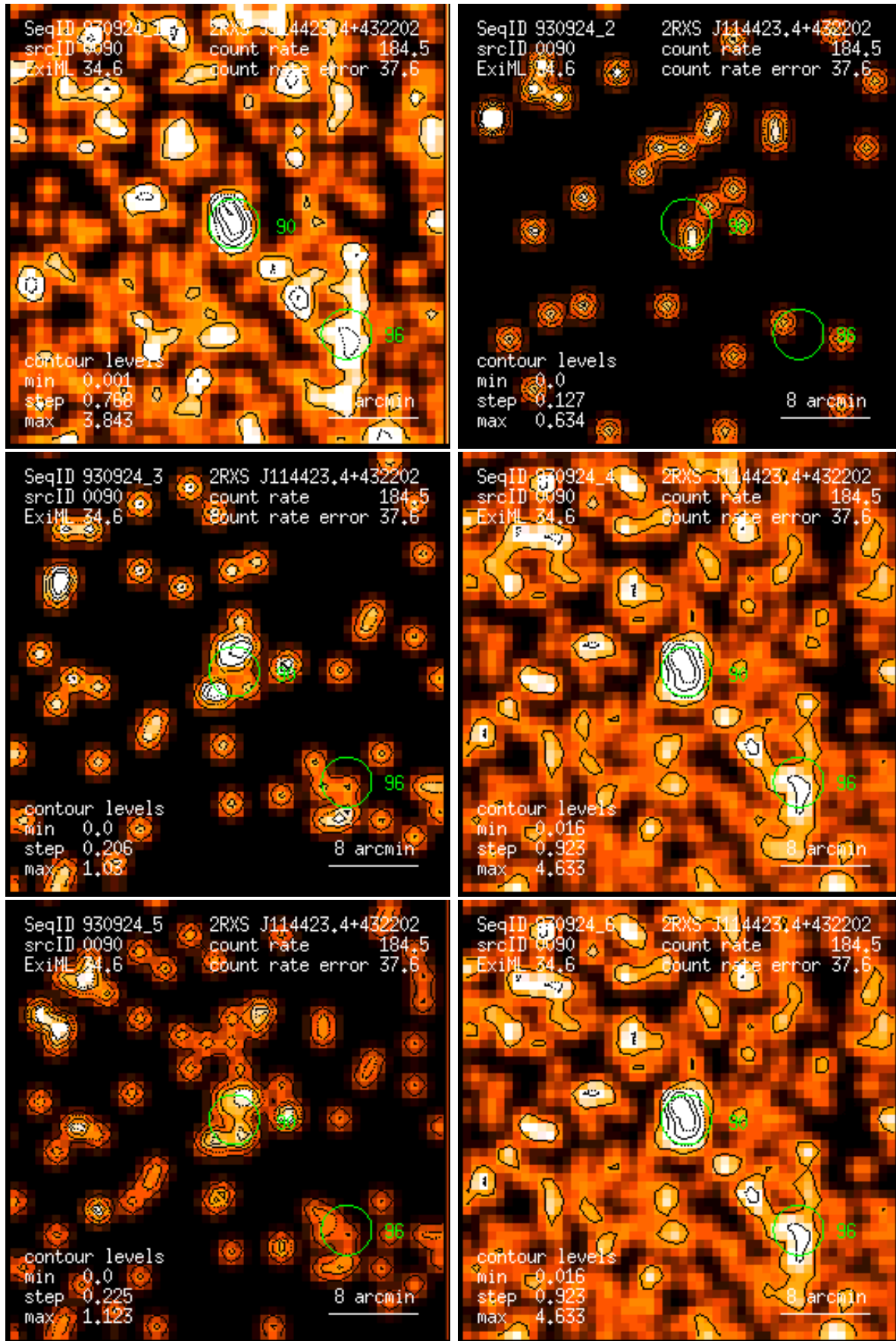
Figure 90: RASS 930924: detection 0090: band rate images, Gaussian filter: (1) PSPC channels 11 – 41, (2) 52 – 90, (3) 91 – 201, (4) 11 – 235, (5) 52 – 201, (6) 11 – 201. Broad band rates in counts/ks. Band rate contour levels in counts/ks/arcmin 2 .
