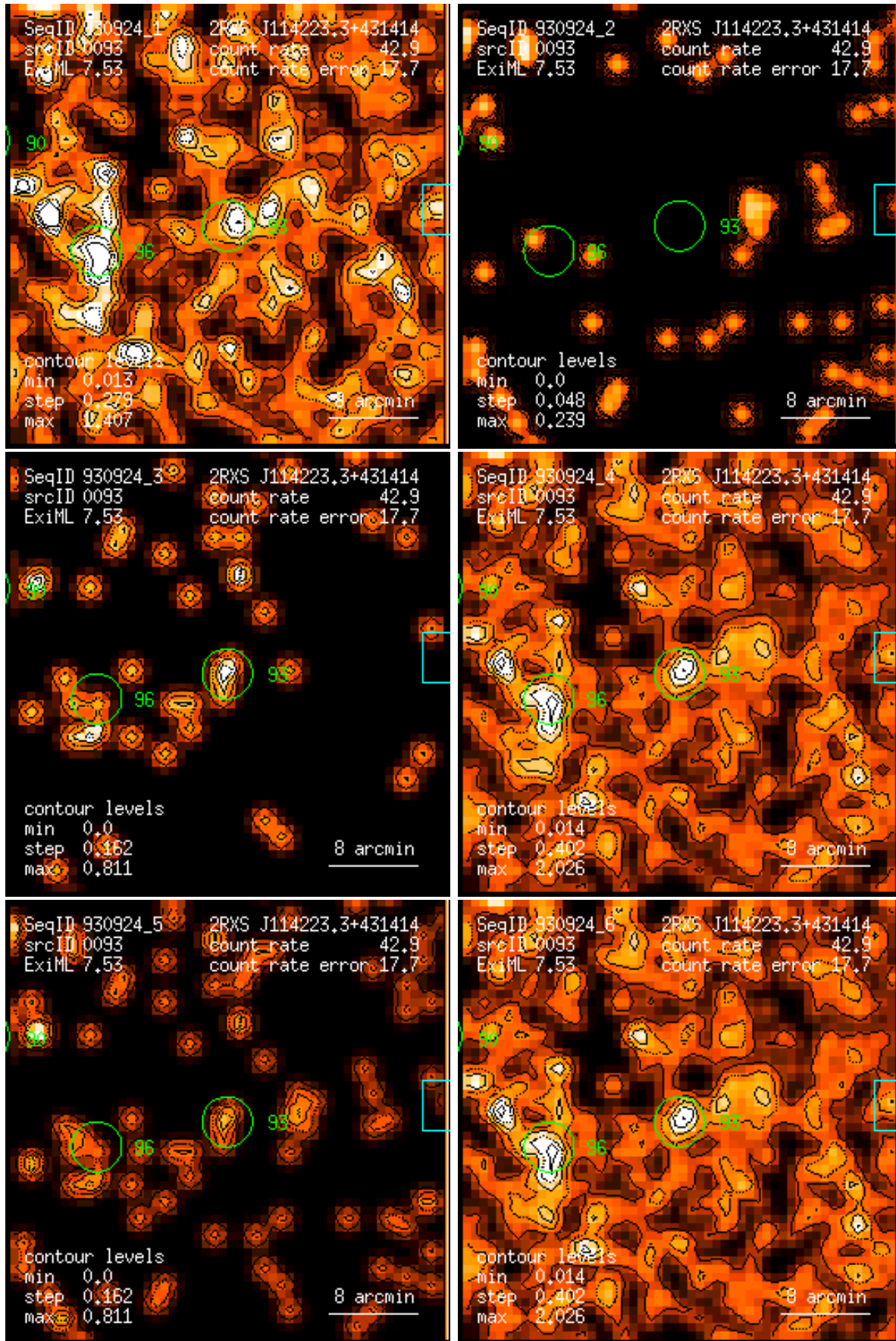
Figure 93: RASS 930924: detection 0093: band rate images, Gaussian filter: (1) PSPC channels 11 – 41, (2) 52 – 90, (3) 91 – 201, (4) 11 – 235, (5) 52 – 201, (6) 11 – 201. Broad band rates in counts/ks. Band rate contour levels in counts/ks/arcmin 2 .
