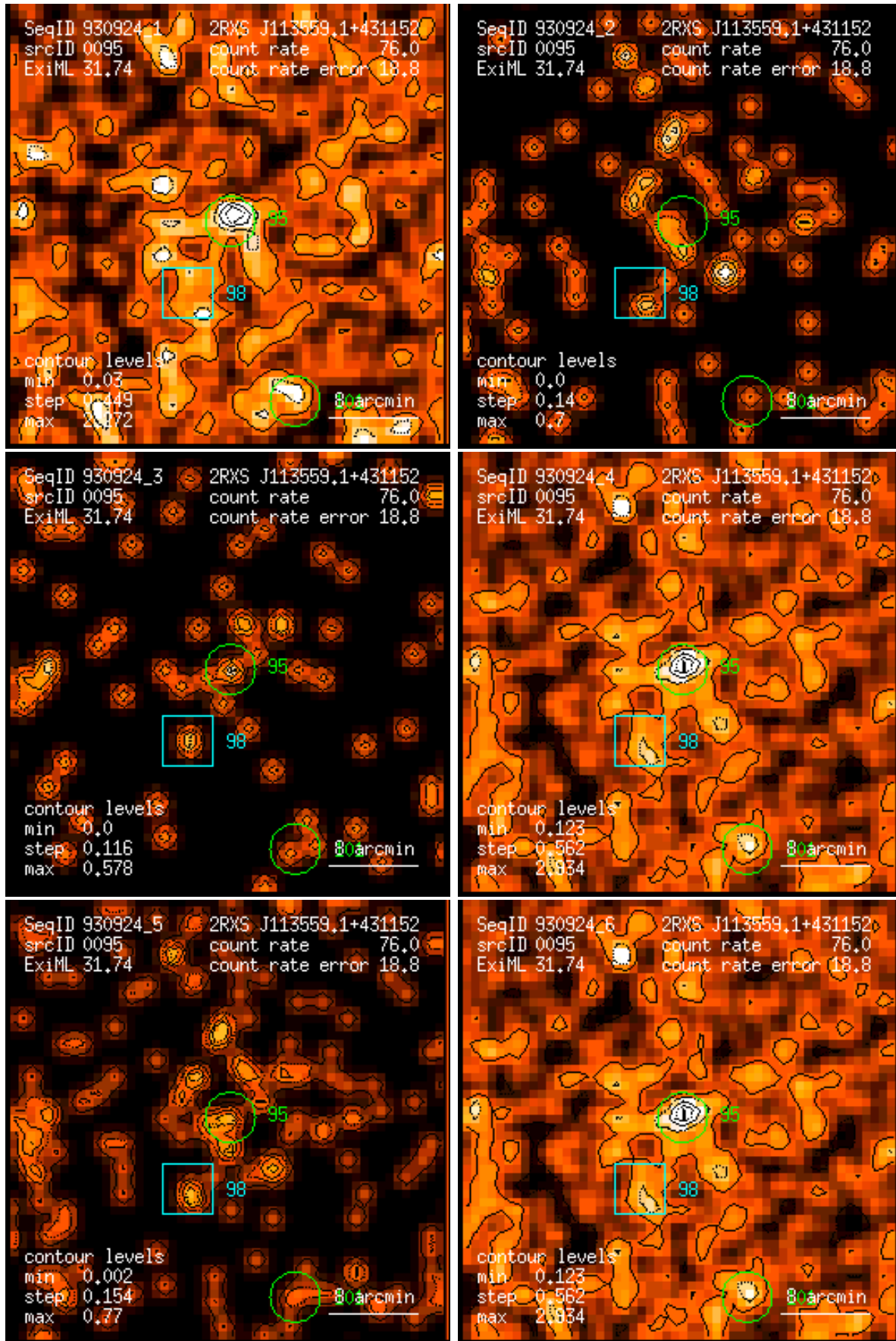
Figure 95: RASS 930924: detection 0095: band rate images, Gaussian filter: (1) PSPC channels 11 – 41, (2) 52 – 90, (3) 91 – 201, (4) 11 – 235, (5) 52 – 201, (6) 11 – 201. Broad band rates in counts/ks. Band rate contour levels in counts/ks/arcmin 2 .
