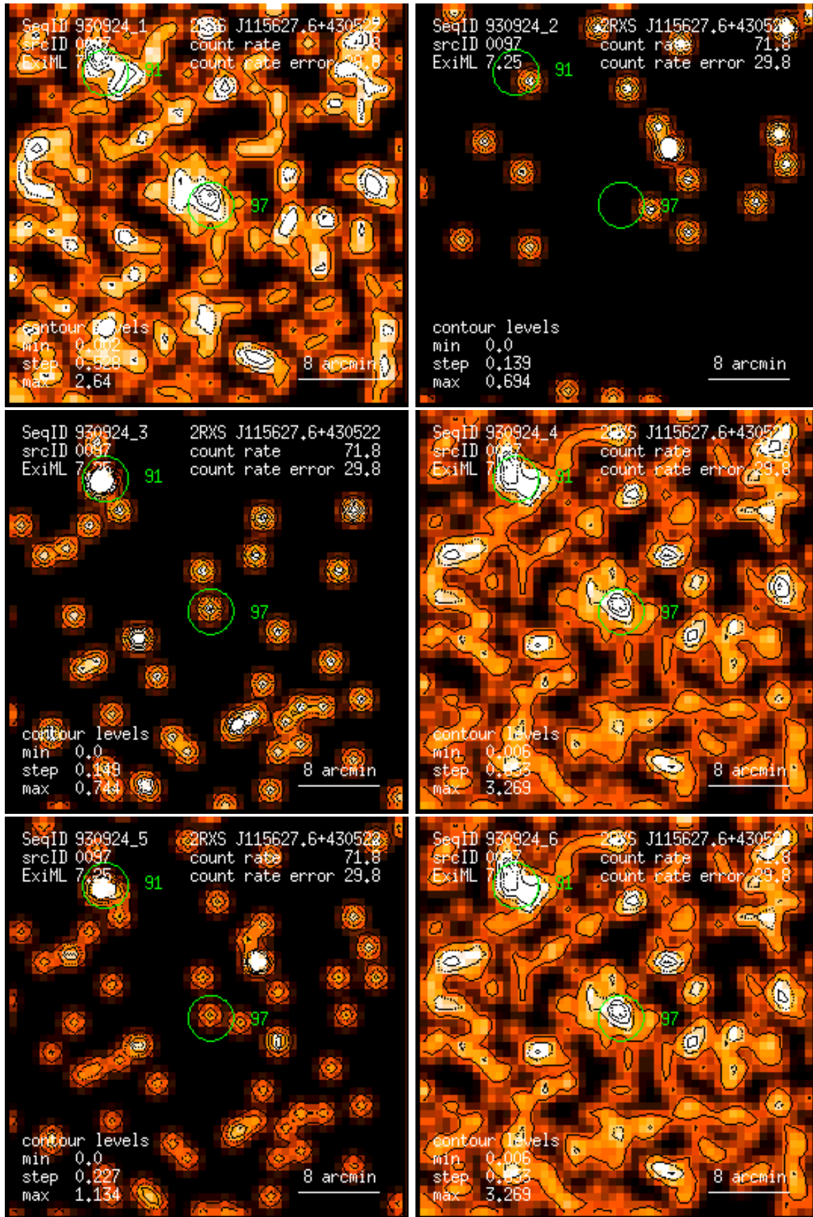
Figure 97: RASS 930924: detection 0097: band rate images, Gaussian filter: (1) PSPC channels 11 – 41, (2) 52 – 90, (3) 91 – 201, (4) 11 – 235, (5) 52 – 201, (6) 11 – 201. Broad band rates in counts/ks. Band rate contour levels in counts/ks/arcmin 2 .
