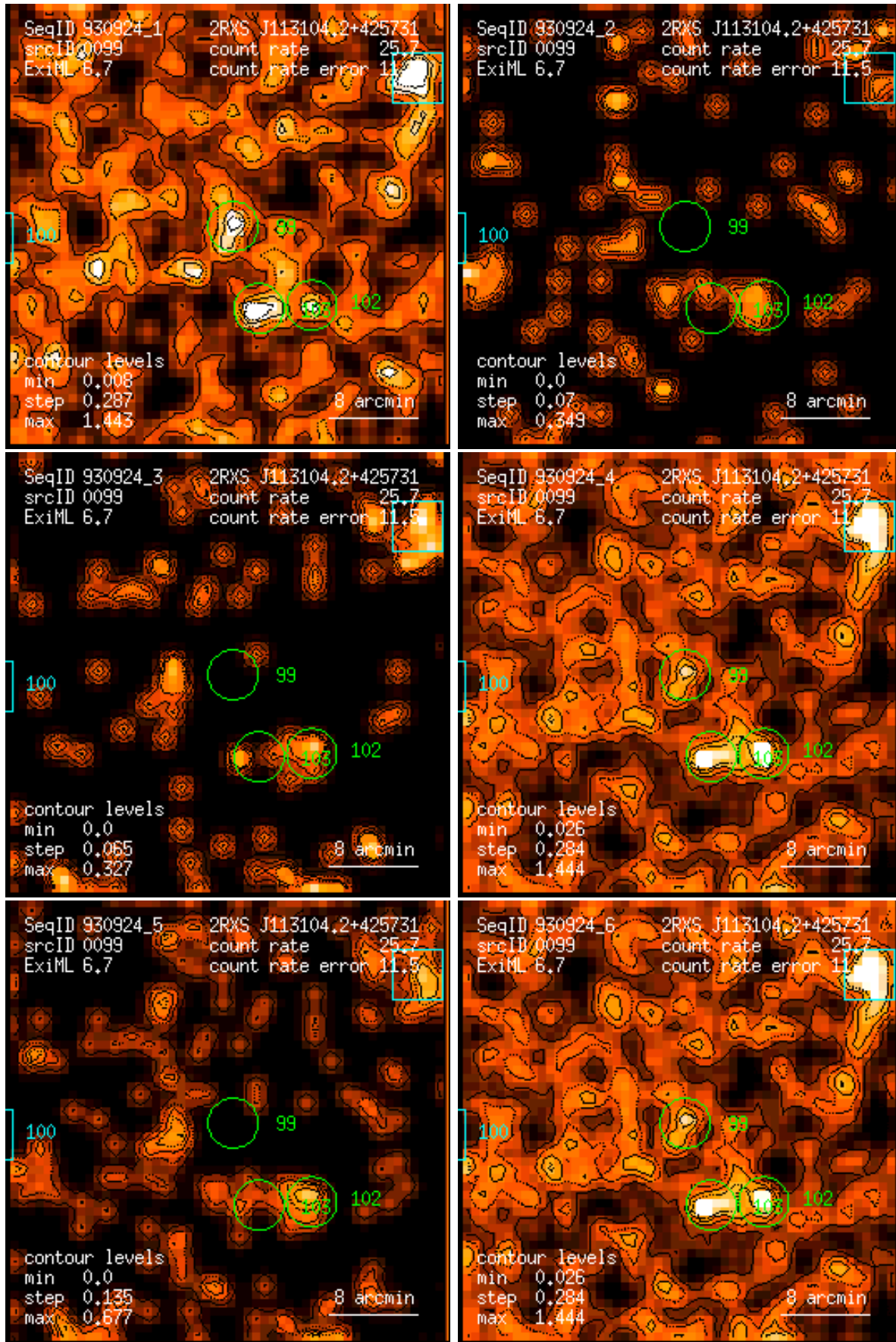
Figure 99: RASS 930924: detection 0099: band rate images, Gaussian filter: (1) PSPC channels 11 – 41, (2) 52 – 90, (3) 91 – 201, (4) 11 – 235, (5) 52 – 201, (6) 11 – 201. Broad band rates in counts/ks. Band rate contour levels in counts/ks/arcmin 2 .
