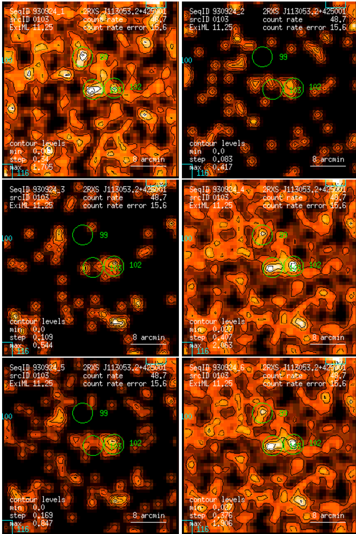
Figure 103: RASS 930924: detection 0103: band rate images, Gaussian filter: (1) PSPC channels 11 – 41, (2) 52 – 90, (3) 91 – 201, (4) 11 – 235, (5) 52 – 201, (6) 11 – 201. Broad band rates in counts/ks. Band rate contour levels in counts/ks/arcmin 2 .
