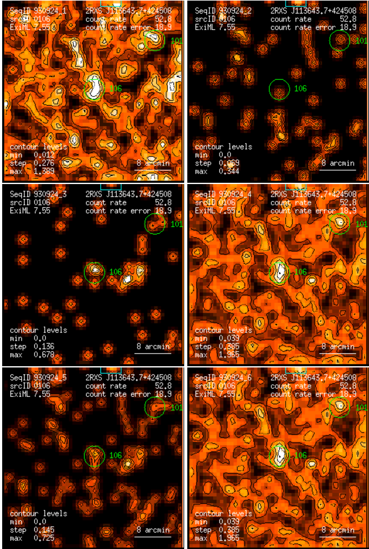
Figure 106: RASS 930924: detection 0106: band rate images, Gaussian filter: (1) PSPC channels 11 – 41, (2) 52 – 90, (3) 91 – 201, (4) 11 – 235, (5) 52 – 201, (6) 11 – 201. Broad band rates in counts/ks. Band rate contour levels in counts/ks/arcmin 2 .
