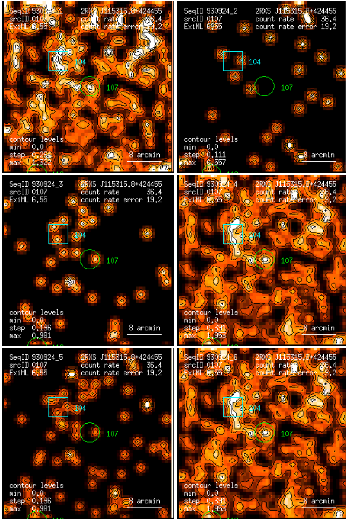
Figure 107: RASS 930924: detection 0107: band rate images, Gaussian filter: (1) PSPC channels 11 – 41, (2) 52 – 90, (3) 91 – 201, (4) 11 – 235, (5) 52 – 201, (6) 11 – 201. Broad band rates in counts/ks. Band rate contour levels in counts/ks/arcmin 2 .
