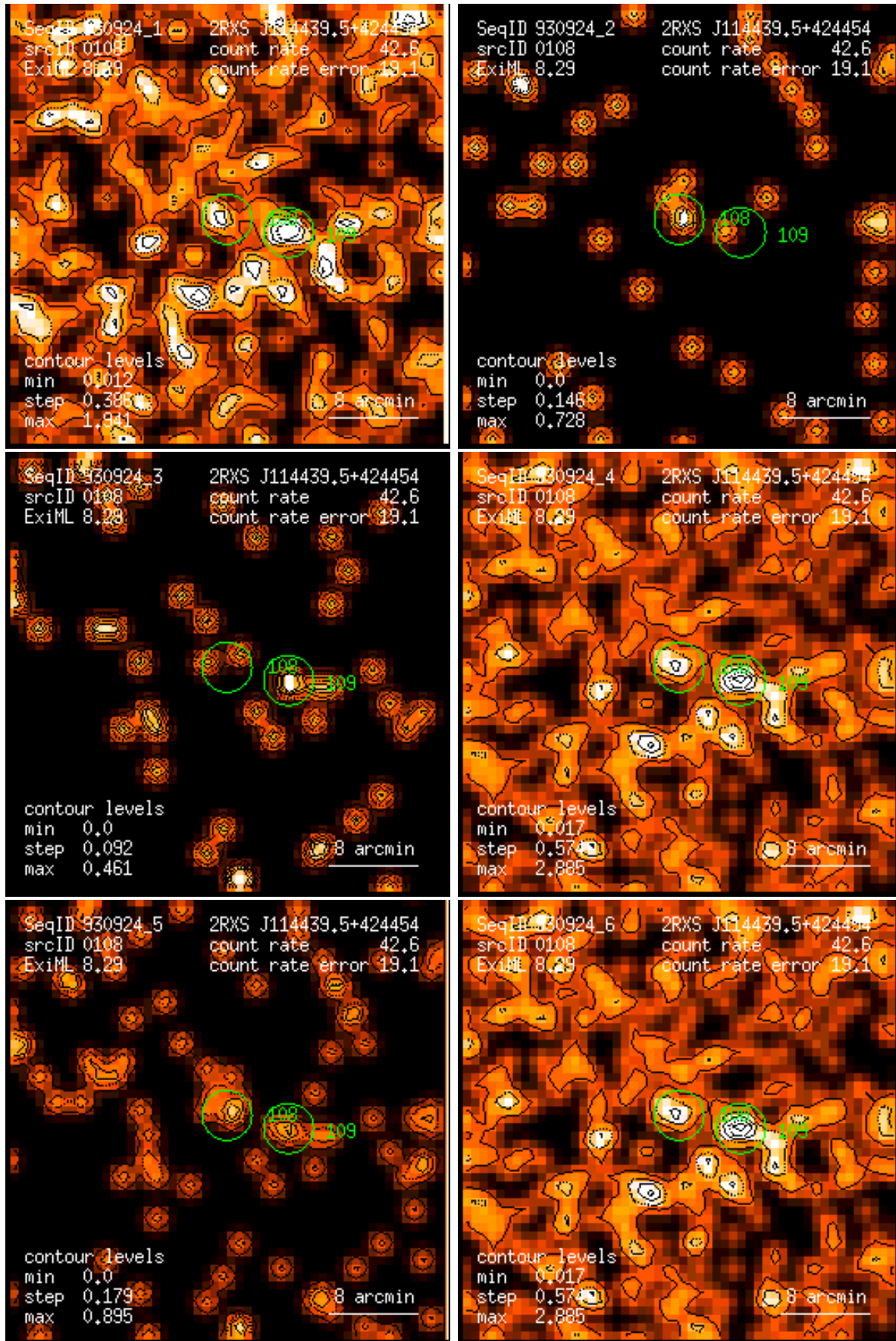
Figure 108: RASS 930924: detection 0108: band rate images, Gaussian filter: (1) PSPC channels 11 – 41, (2) 52 – 90, (3) 91 – 201, (4) 11 – 235, (5) 52 – 201, (6) 11 – 201. Broad band rates in counts/ks. Band rate contour levels in counts/ks/arcmin 2 .
