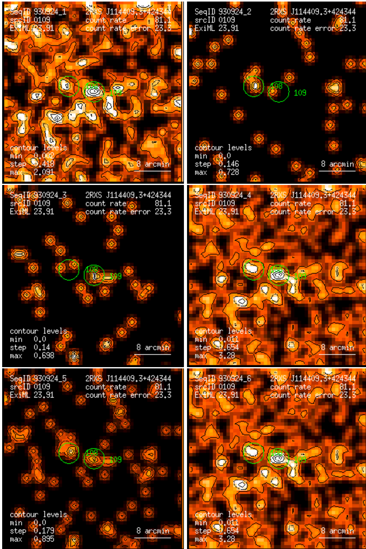
Figure 109: RASS 930924: detection 0109: band rate images, Gaussian filter: (1) PSPC channels 11 – 41, (2) 52 – 90, (3) 91 – 201, (4) 11 – 235, (5) 52 – 201, (6) 11 – 201. Broad band rates in counts/ks. Band rate contour levels in counts/ks/arcmin 2 .
