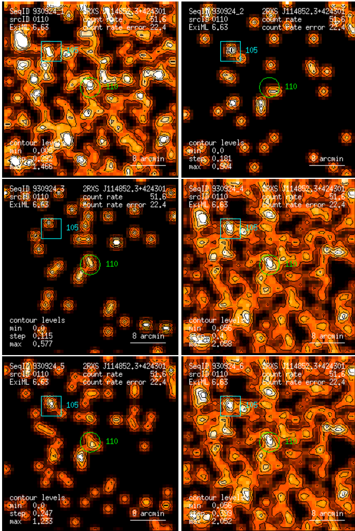
Figure 110: RASS 930924: detection 0110: band rate images, Gaussian filter: (1) PSPC channels 11 – 41, (2) 52 – 90, (3) 91 – 201, (4) 11 – 235, (5) 52 – 201, (6) 11 – 201. Broad band rates in counts/ks. Band rate contour levels in counts/ks/arcmin 2 .
