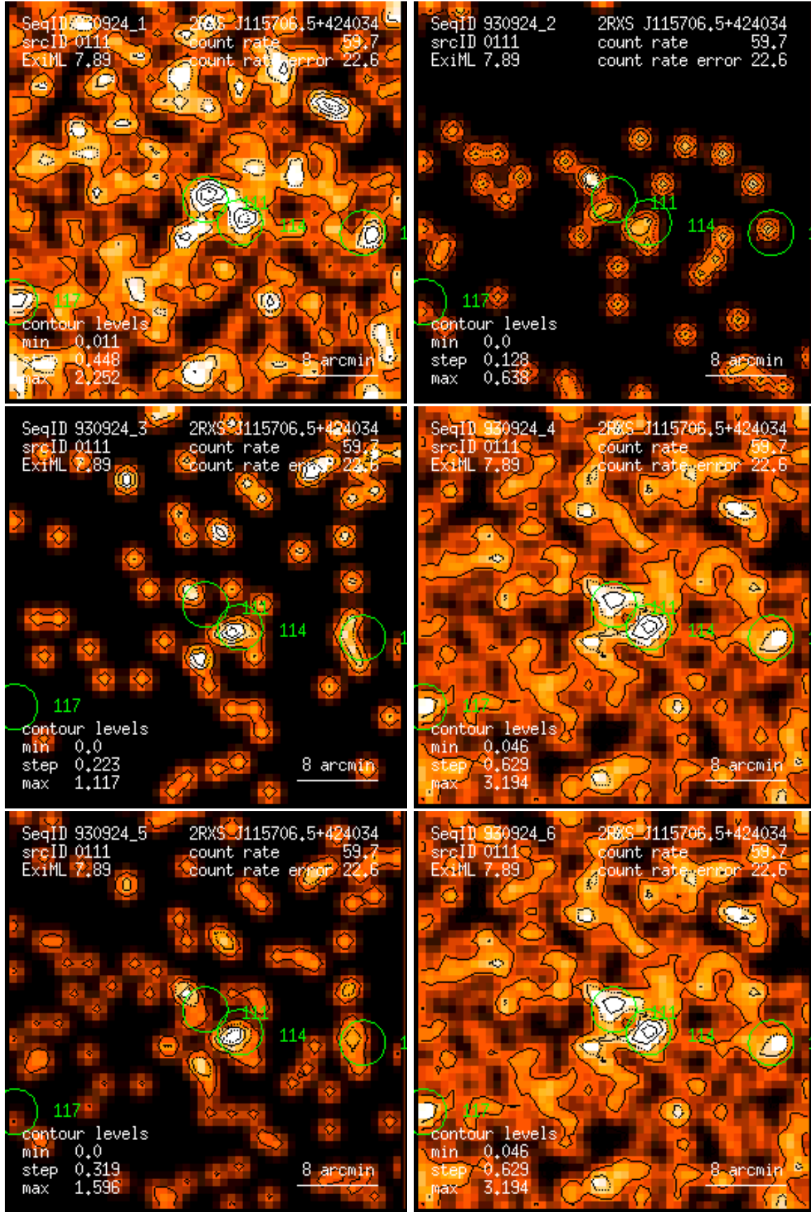
Figure 111: RASS 930924: detection 0111: band rate images, Gaussian filter: (1) PSPC channels 11 – 41, (2) 52 – 90, (3) 91 – 201, (4) 11 – 235, (5) 52 – 201, (6) 11 – 201. Broad band rates in counts/ks. Band rate contour levels in counts/ks/arcmin 2 .
