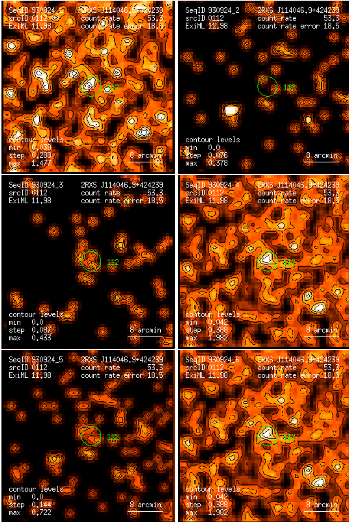
Figure 112: RASS 930924: detection 0112: band rate images, Gaussian filter: (1) PSPC channels 11 – 41, (2) 52 – 90, (3) 91 – 201, (4) 11 – 235, (5) 52 – 201, (6) 11 – 201. Broad band rates in counts/ks. Band rate contour levels in counts/ks/arcmin 2 .
