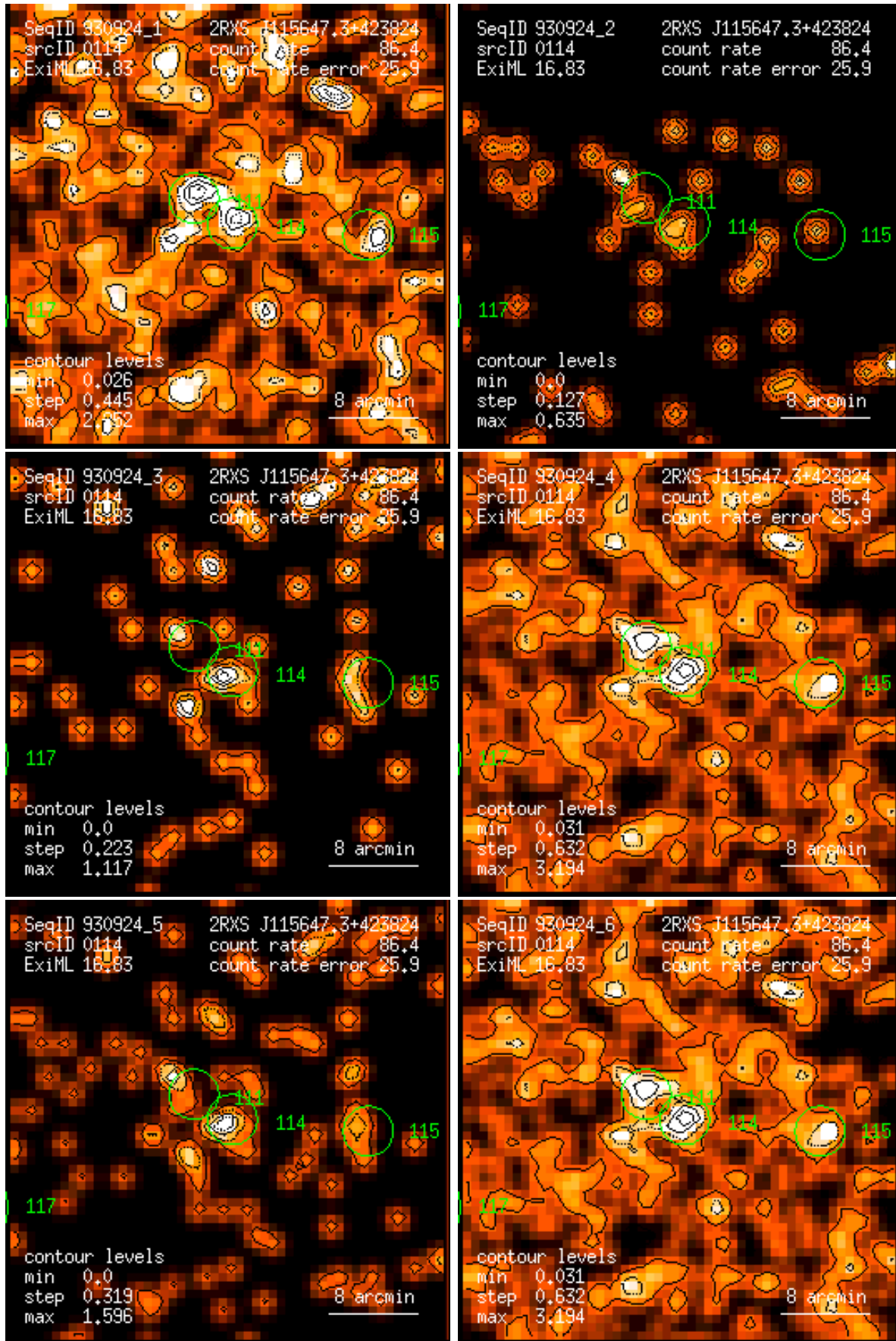
Figure 114: RASS 930924: detection 0114: band rate images, Gaussian filter: (1) PSPC channels 11 – 41, (2) 52 – 90, (3) 91 – 201, (4) 11 – 235, (5) 52 – 201, (6) 11 – 201. Broad band rates in counts/ks. Band rate contour levels in counts/ks/arcmin 2 .
