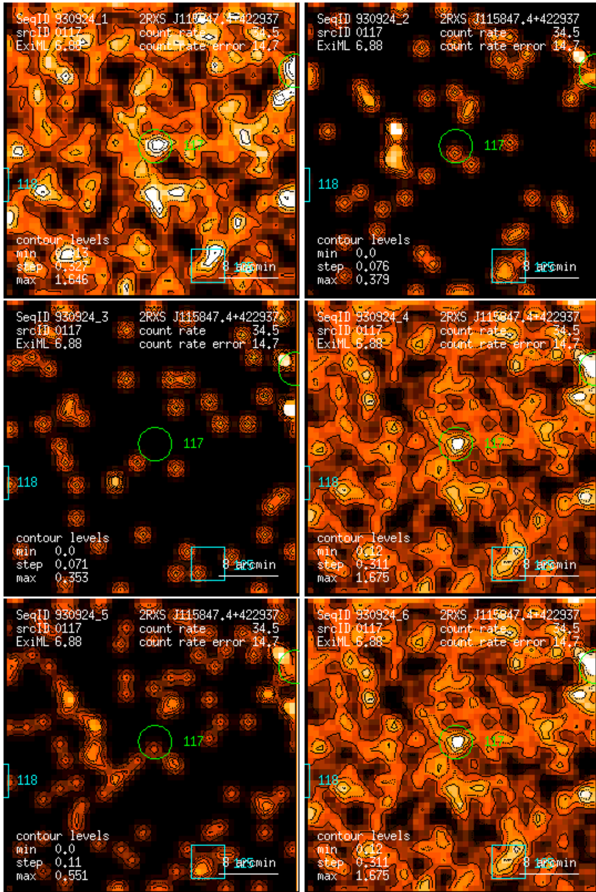
Figure 117: RASS 930924: detection 0117: band rate images, Gaussian filter: (1) PSPC channels 11 – 41, (2) 52 – 90, (3) 91 – 201, (4) 11 – 235, (5) 52 – 201, (6) 11 – 201. Broad band rates in counts/ks. Band rate contour levels in counts/ks/arcmin 2 .
