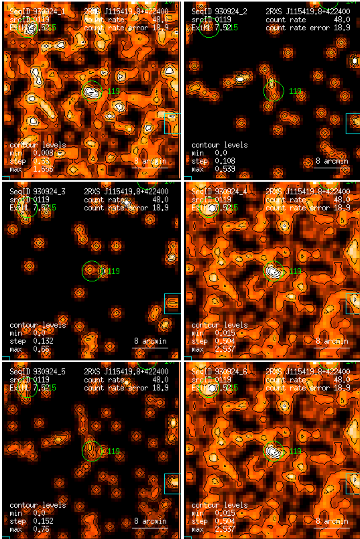
Figure 119: RASS 930924: detection 0119: band rate images, Gaussian filter: (1) PSPC channels 11 – 41, (2) 52 – 90, (3) 91 – 201, (4) 11 – 235, (5) 52 – 201, (6) 11 – 201. Broad band rates in counts/ks. Band rate contour levels in counts/ks/arcmin 2 .
