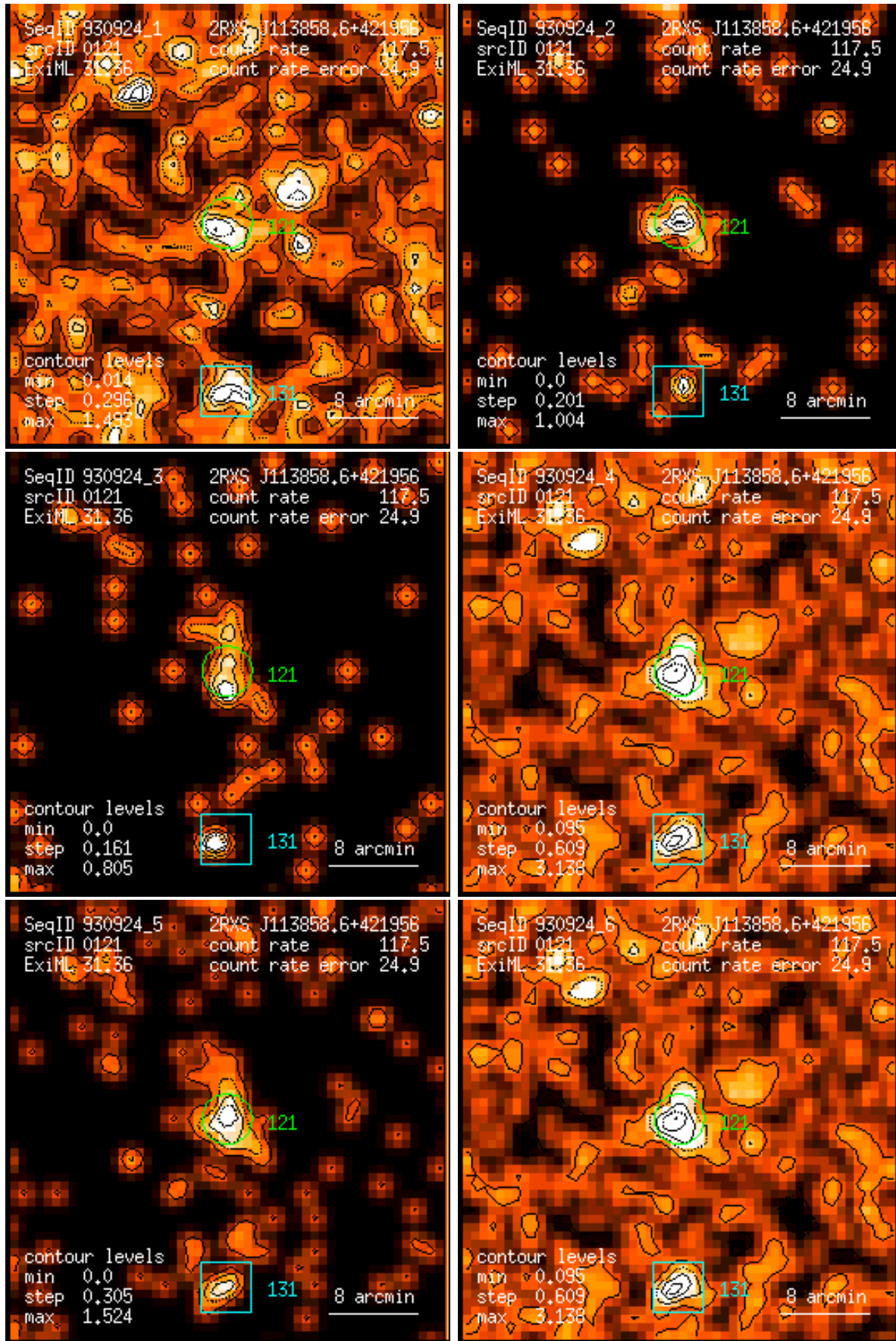
Figure 121: RASS 930924: detection 0121: band rate images, Gaussian filter: (1) PSPC channels 11 – 41, (2) 52 – 90, (3) 91 – 201, (4) 11 – 235, (5) 52 – 201, (6) 11 – 201. Broad band rates in counts/ks. Band rate contour levels in counts/ks/arcmin 2 .
