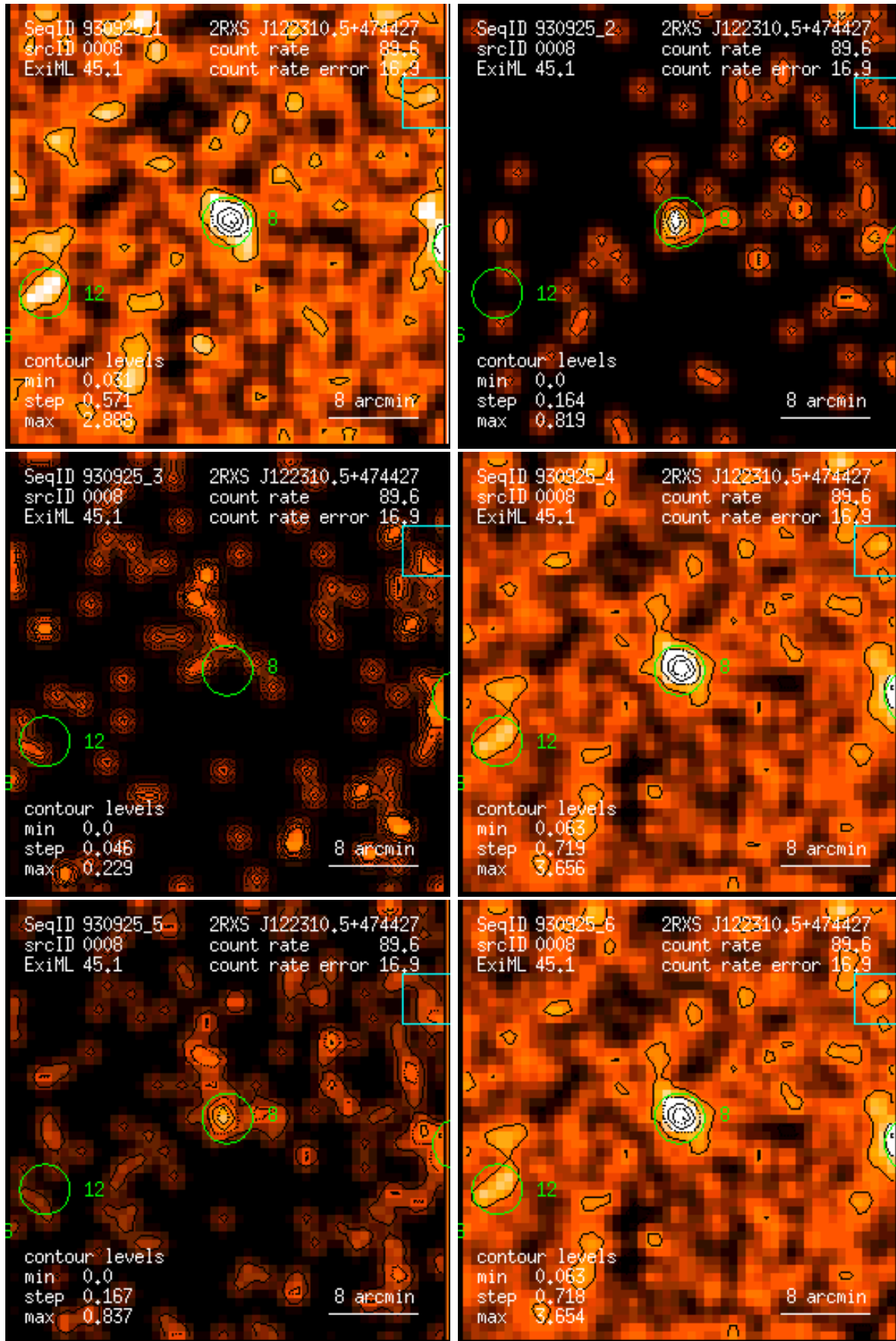
Figure 8: RASS 930925: detection 0008: band rate images, Gaussian filter: (1) PSPC channels 11 – 41, (2) 52 – 90, (3) 91 – 201, (4) 11 – 235, (5) 52 – 201, (6) 11 – 201. Broad band rates in counts/ks. Band rate contour levels in counts/ks/arcmin 2 .
