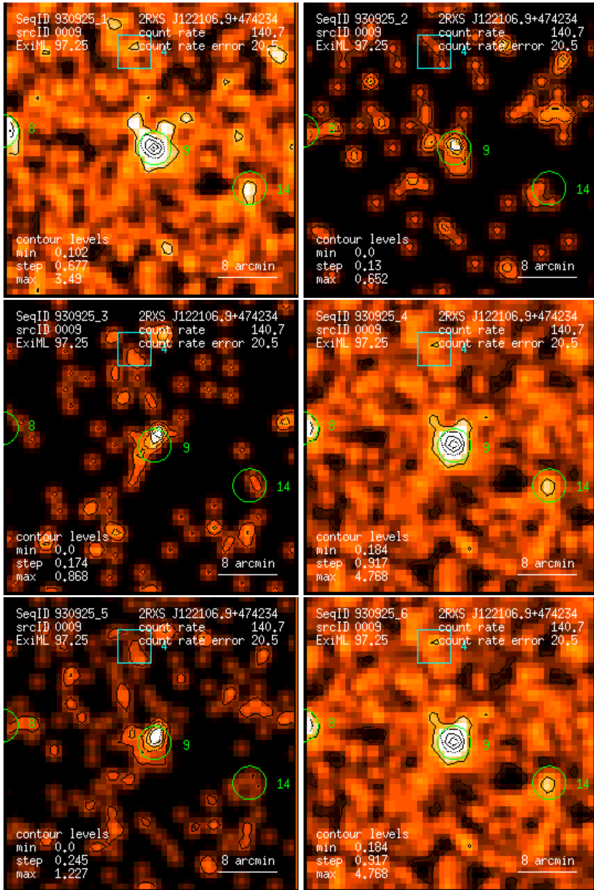
Figure 9: RASS 930925: detection 0009: band rate images, Gaussian filter: (1) PSPC channels 11 – 41, (2) 52 – 90, (3) 91 – 201, (4) 11 – 235, (5) 52 – 201, (6) 11 – 201. Broad band rates in counts/ks. Band rate contour levels in counts/ks/arcmin 2 .
