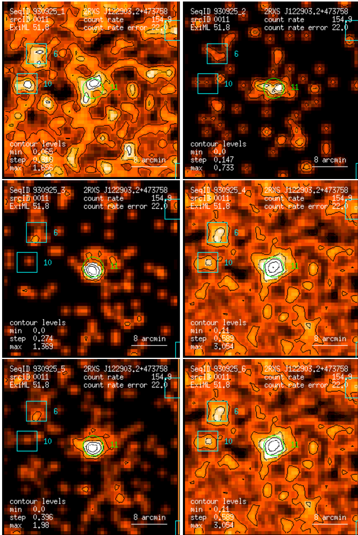
Figure 11: RASS 930925: detection 0011: band rate images, Gaussian filter: (1) PSPC channels 11 – 41, (2) 52 – 90, (3) 91 – 201, (4) 11 – 235, (5) 52 – 201, (6) 11 – 201. Broad band rates in counts/ks. Band rate contour levels in counts/ks/arcmin 2 .
