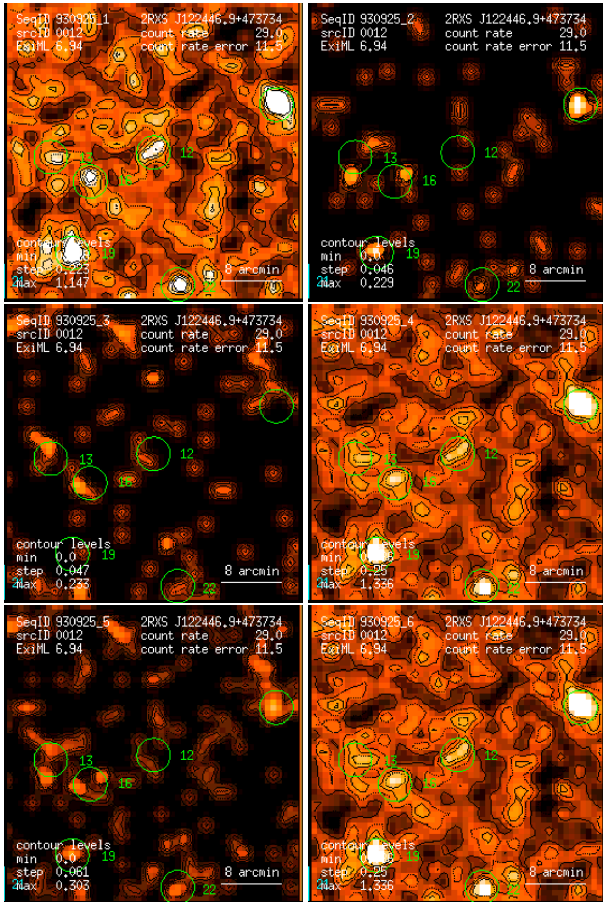
Figure 12: RASS 930925: detection 0012: band rate images, Gaussian filter: (1) PSPC channels 11 – 41, (2) 52 – 90, (3) 91 – 201, (4) 11 – 235, (5) 52 – 201, (6) 11 – 201. Broad band rates in counts/ks. Band rate contour levels in counts/ks/arcmin 2 .
