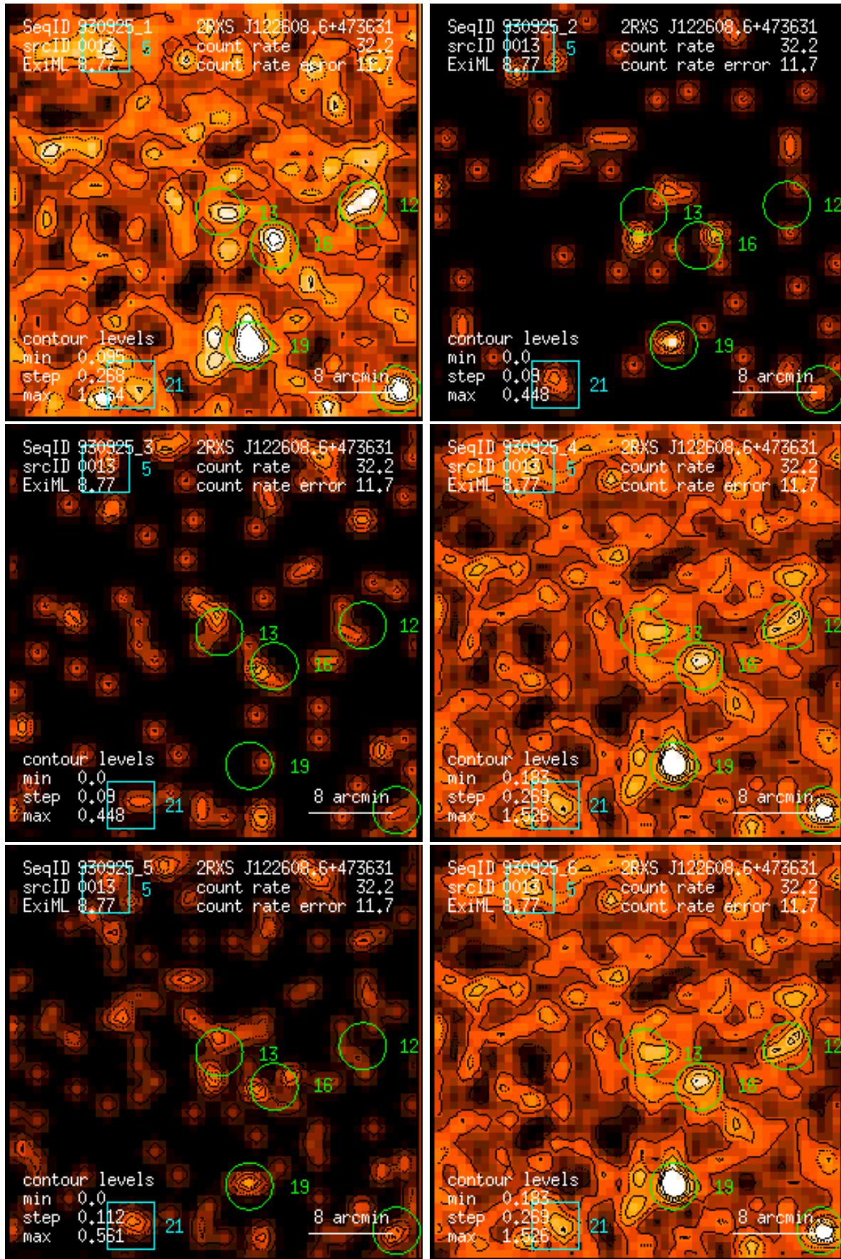
Figure 13: RASS 930925: detection 0013: band rate images, Gaussian filter: (1) PSPC channels 11 – 41, (2) 52 – 90, (3) 91 – 201, (4) 11 – 235, (5) 52 – 201, (6) 11 – 201. Broad band rates in counts/ks. Band rate contour levels in counts/ks/arcmin 2 .
