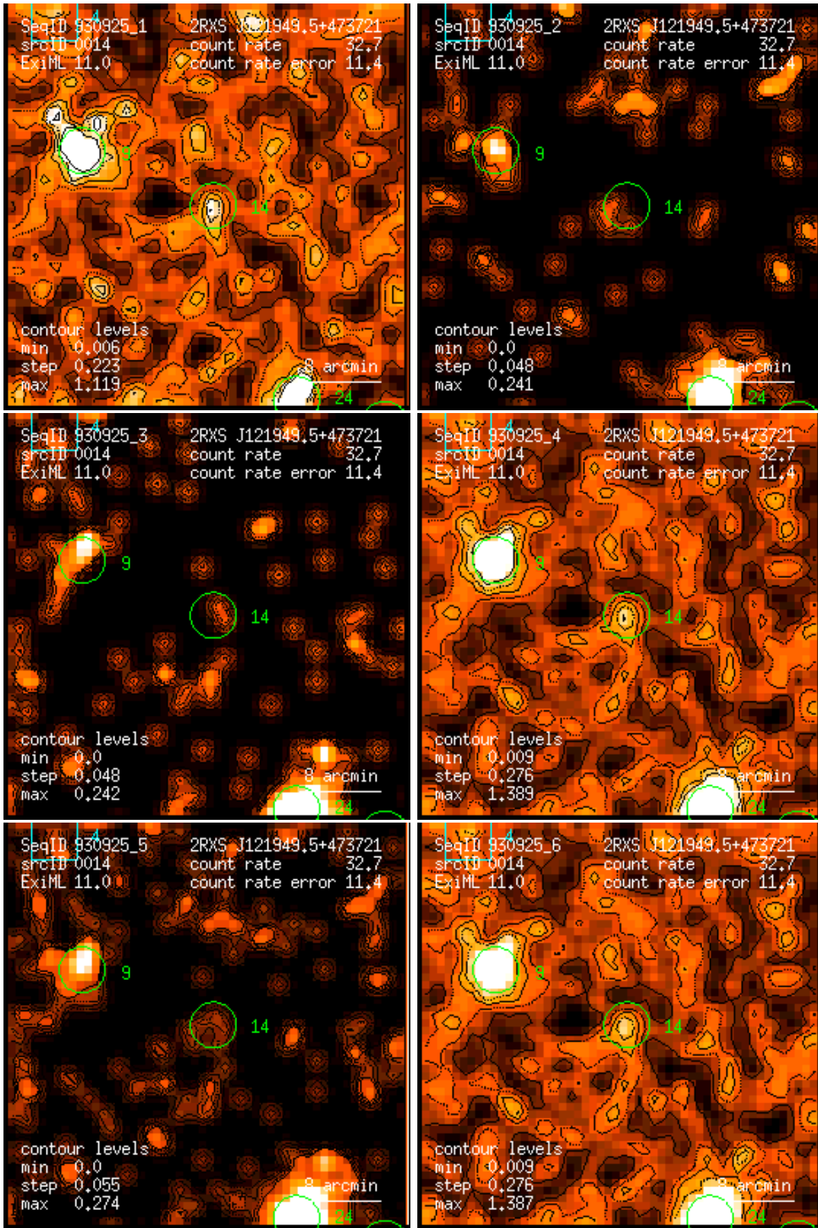
Figure 14: RASS 930925: detection 0014: band rate images, Gaussian filter: (1) PSPC channels 11 – 41, (2) 52 – 90, (3) 91 – 201, (4) 11 – 235, (5) 52 – 201, (6) 11 – 201. Broad band rates in counts/ks. Band rate contour levels in counts/ks/arcmin 2 .
