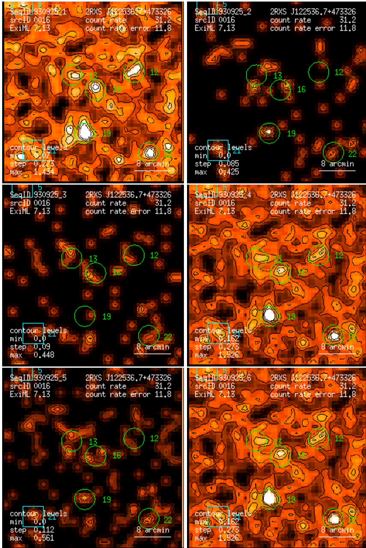
Figure 16: RASS 930925: detection 0016: band rate images, Gaussian filter: (1) PSPC channels 11 – 41, (2) 52 – 90, (3) 91 – 201, (4) 11 – 235, (5) 52 – 201, (6) 11 – 201. Broad band rates in counts/ks. Band rate contour levels in counts/ks/arcmin 2 .
