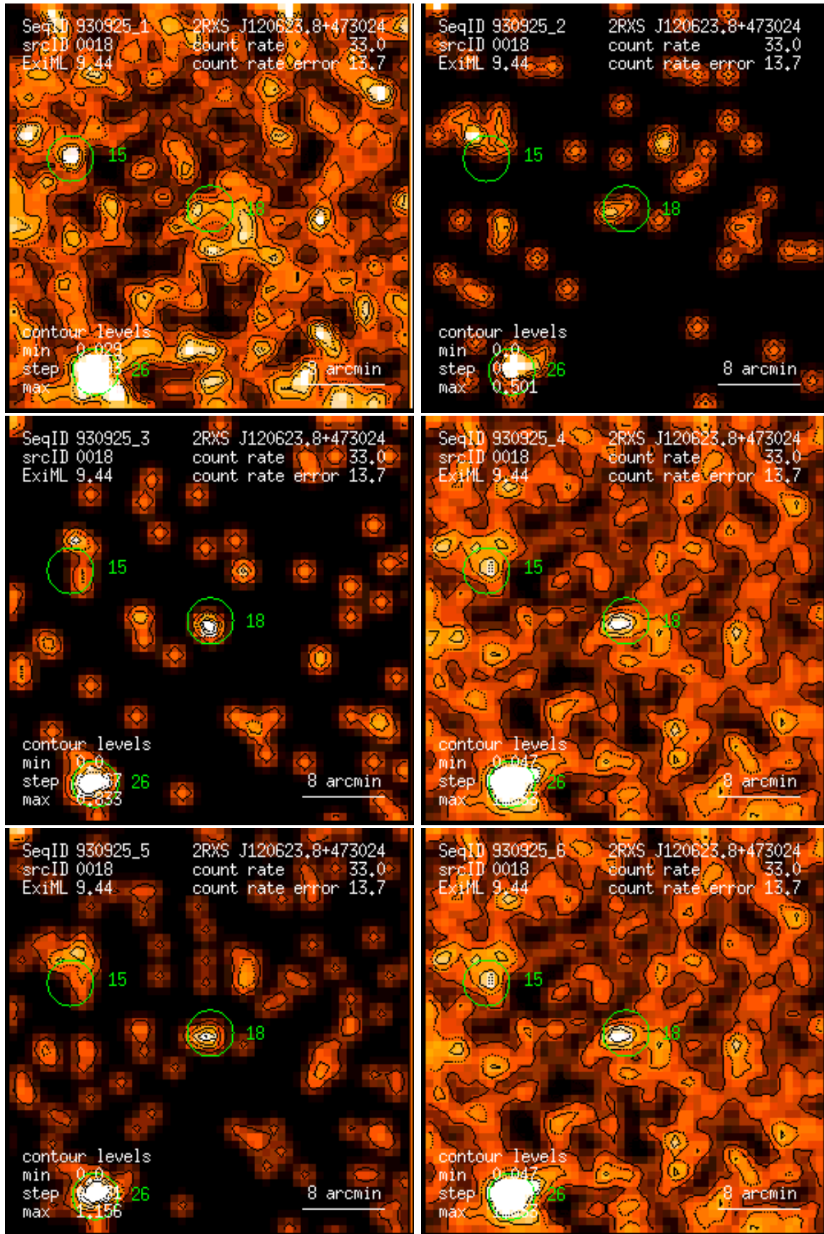
Figure 18: RASS 930925: detection 0018: band rate images, Gaussian filter: (1) PSPC channels 11 – 41, (2) 52 – 90, (3) 91 – 201, (4) 11 – 235, (5) 52 – 201, (6) 11 – 201. Broad band rates in counts/ks. Band rate contour levels in counts/ks/arcmin 2 .
