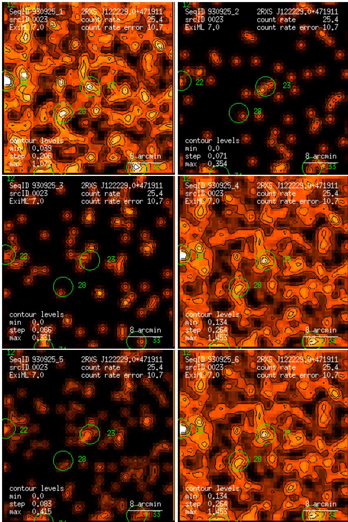
Figure 23: RASS 930925: detection 0023: band rate images, Gaussian filter: (1) PSPC channels 11 – 41, (2) 52 – 90, (3) 91 – 201, (4) 11 – 235, (5) 52 – 201, (6) 11 – 201. Broad band rates in counts/ks. Band rate contour levels in counts/ks/arcmin 2 .
