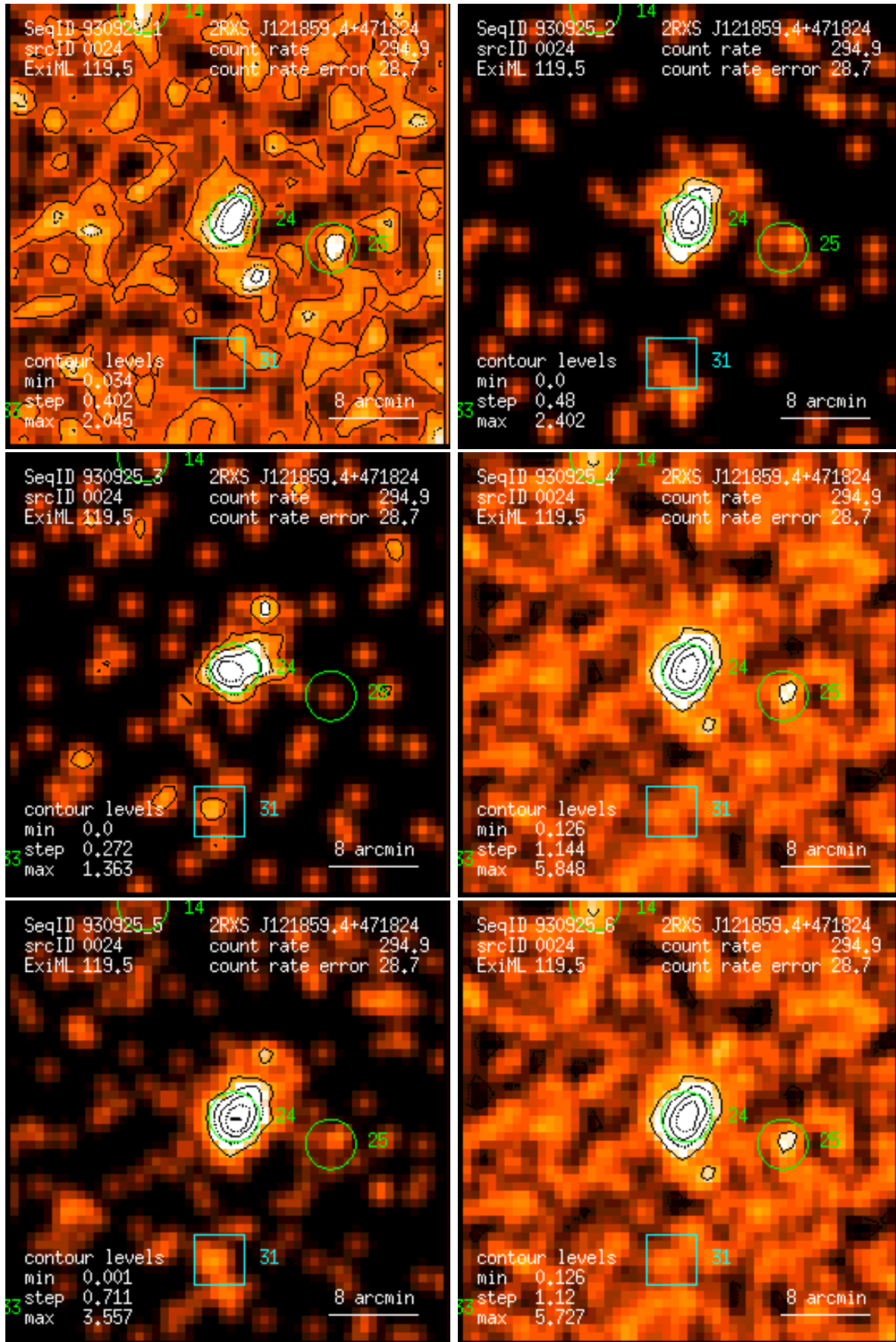
Figure 24: RASS 930925: detection 0024: band rate images, Gaussian filter: (1) PSPC channels 11 – 41, (2) 52 – 90, (3) 91 – 201, (4) 11 – 235, (5) 52 – 201, (6) 11 – 201. Broad band rates in counts/ks. Band rate contour levels in counts/ks/arcmin 2 .
