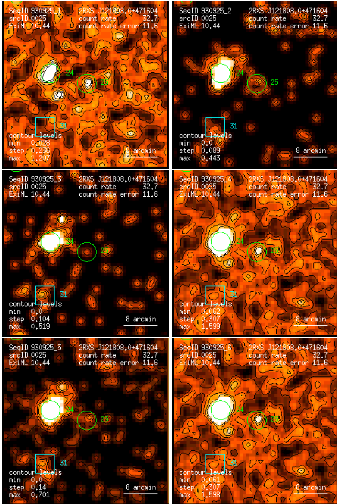
Figure 25: RASS 930925: detection 0025: band rate images, Gaussian filter: (1) PSPC channels 11 – 41, (2) 52 – 90, (3) 91 – 201, (4) 11 – 235, (5) 52 – 201, (6) 11 – 201. Broad band rates in counts/ks. Band rate contour levels in counts/ks/arcmin 2 .
