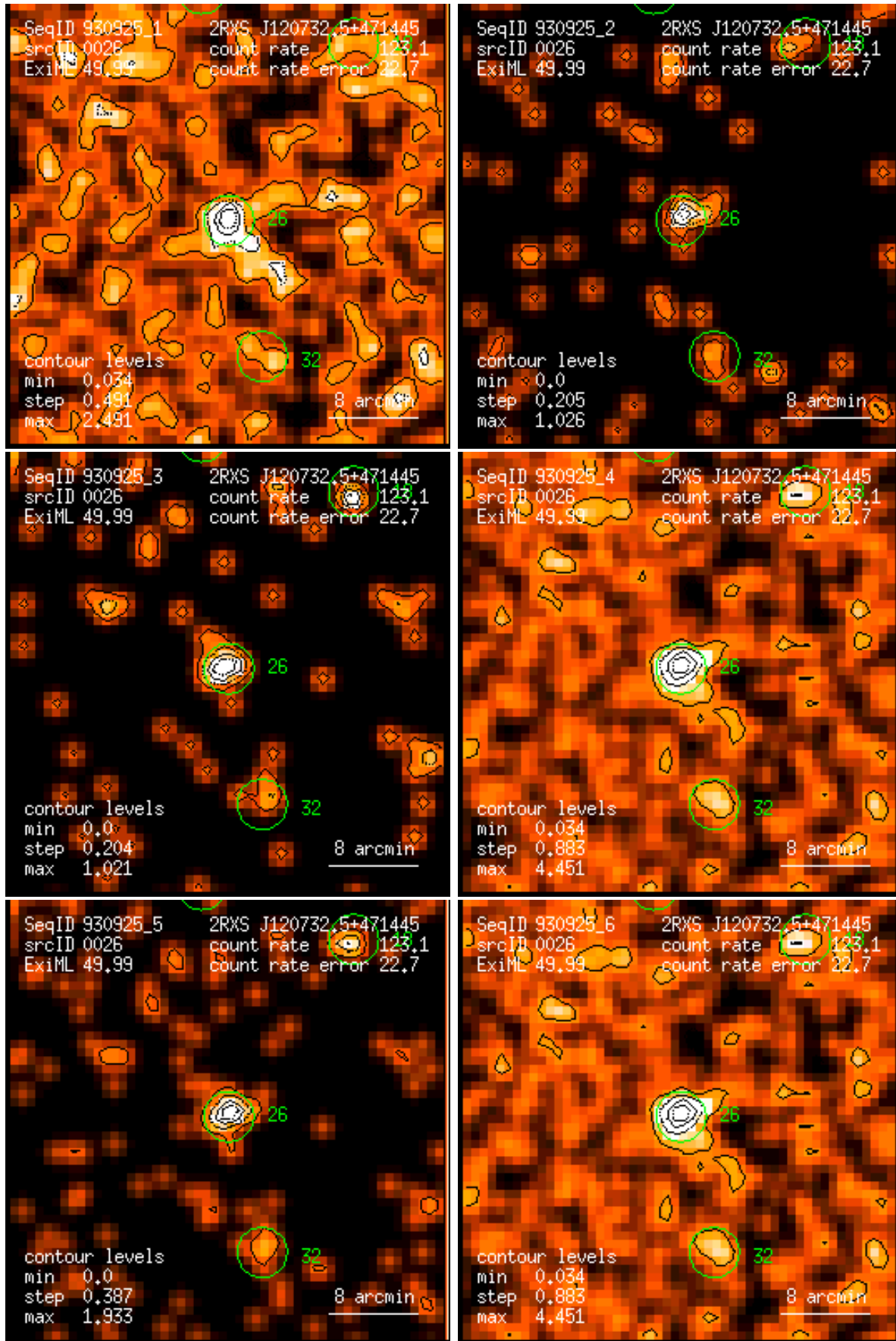
Figure 26: RASS 930925: detection 0026: band rate images, Gaussian filter: (1) PSPC channels 11 – 41, (2) 52 – 90, (3) 91 – 201, (4) 11 – 235, (5) 52 – 201, (6) 11 – 201. Broad band rates in counts/ks. Band rate contour levels in counts/ks/arcmin 2 .
