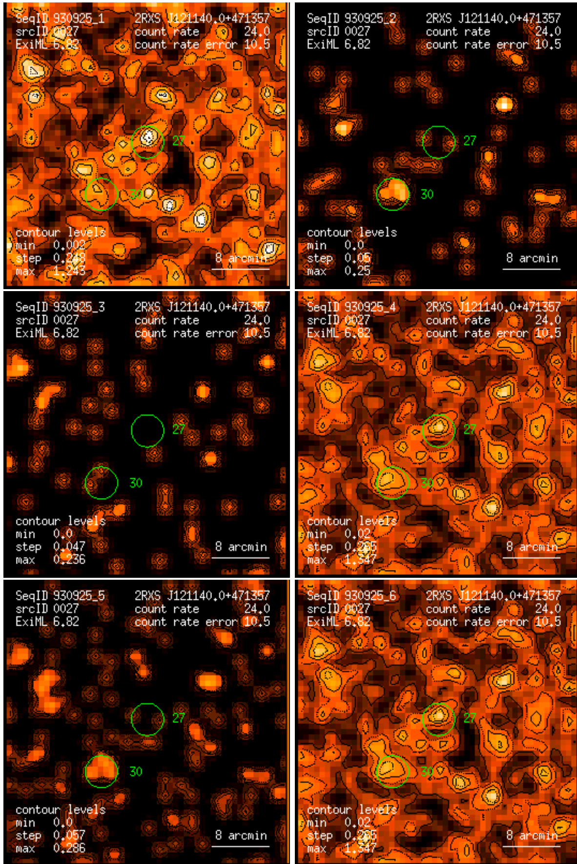
Figure 27: RASS 930925: detection 0027: band rate images, Gaussian filter: (1) PSPC channels 11 – 41, (2) 52 – 90, (3) 91 – 201, (4) 11 – 235, (5) 52 – 201, (6) 11 – 201. Broad band rates in counts/ks. Band rate contour levels in counts/ks/arcmin 2 .
