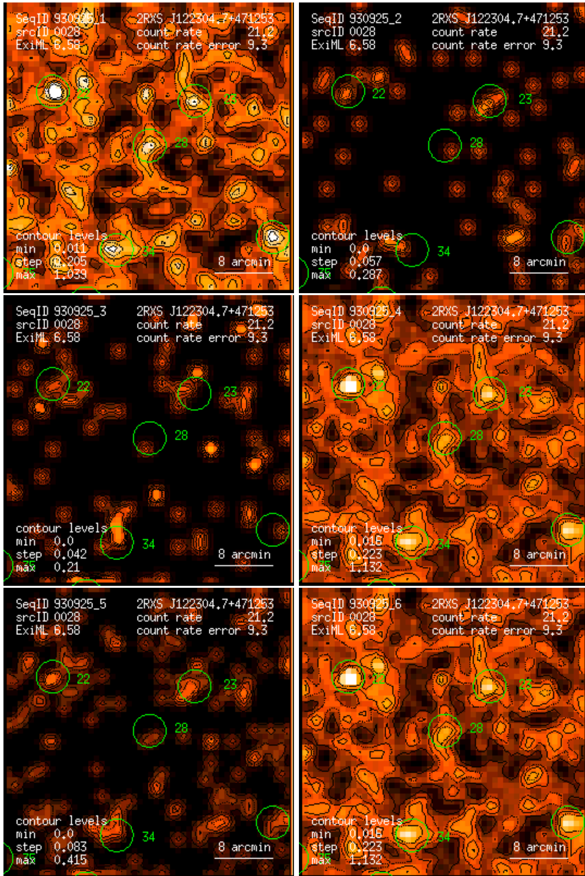
Figure 28: RASS 930925: detection 0028: band rate images, Gaussian filter: (1) PSPC channels 11 – 41, (2) 52 – 90, (3) 91 – 201, (4) 11 – 235, (5) 52 – 201, (6) 11 – 201. Broad band rates in counts/ks. Band rate contour levels in counts/ks/arcmin 2 .
