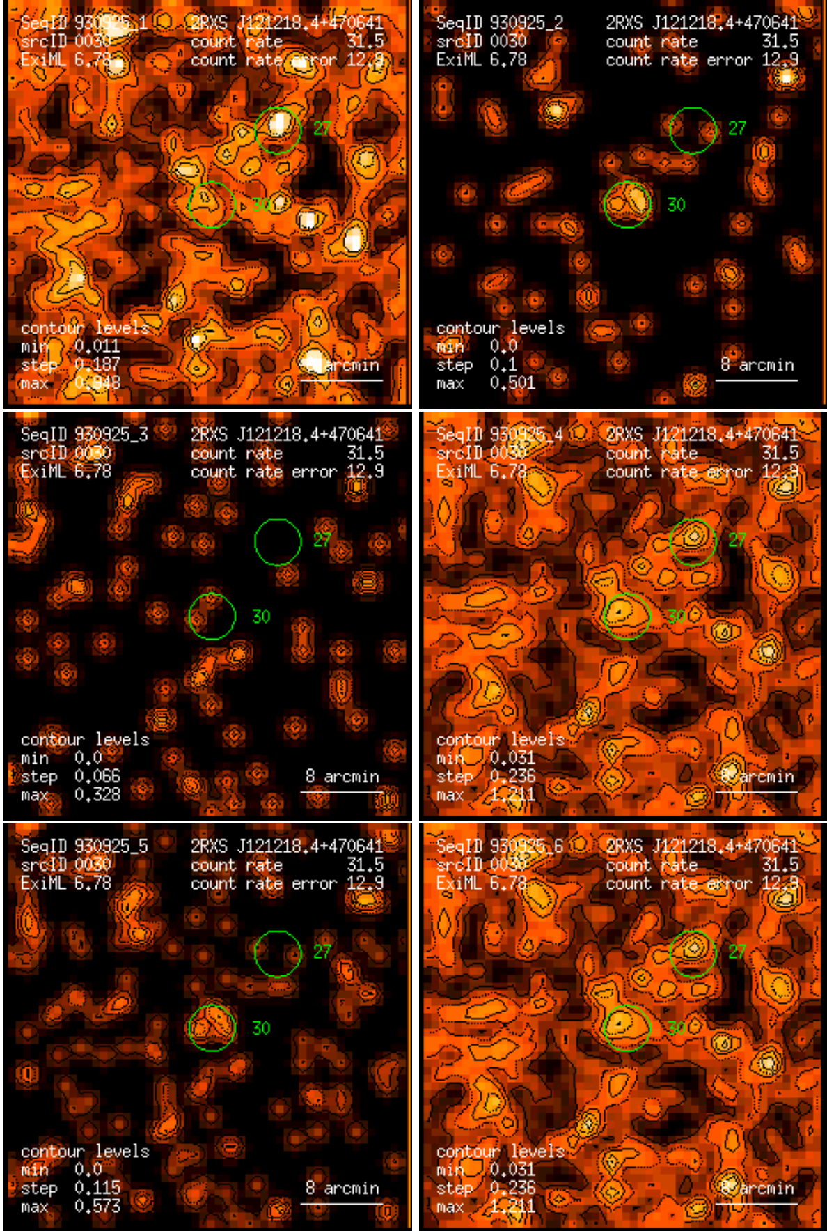
Figure 30: RASS 930925: detection 0030: band rate images, Gaussian filter: (1) PSPC channels 11 – 41, (2) 52 – 90, (3) 91 – 201, (4) 11 – 235, (5) 52 – 201, (6) 11 – 201. Broad band rates in counts/ks. Band rate contour levels in counts/ks/arcmin 2 .
