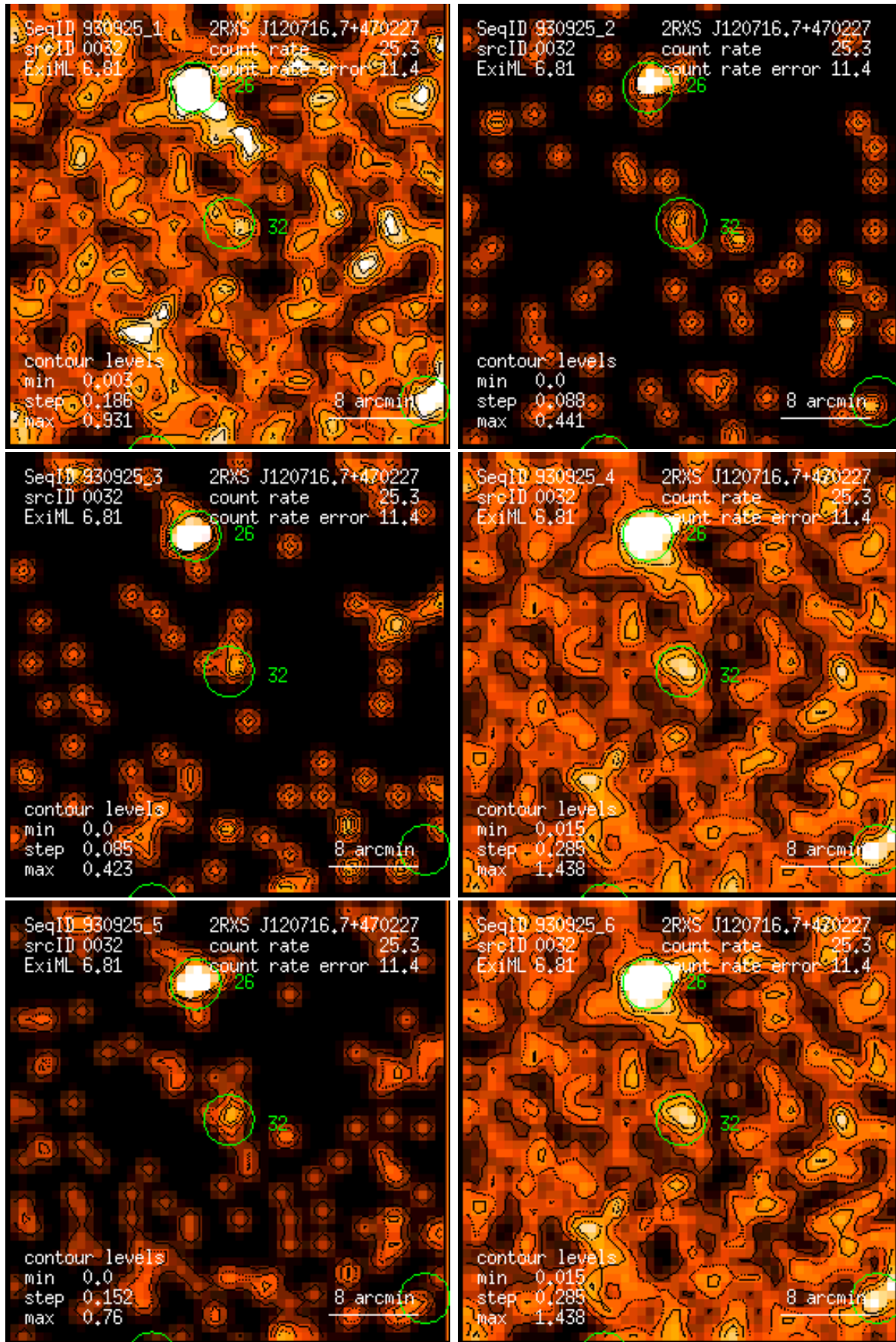
Figure 32: RASS 930925: detection 0032: band rate images, Gaussian filter: (1) PSPC channels 11 – 41, (2) 52 – 90, (3) 91 – 201, (4) 11 – 235, (5) 52 – 201, (6) 11 – 201. Broad band rates in counts/ks. Band rate contour levels in counts/ks/arcmin 2 .
