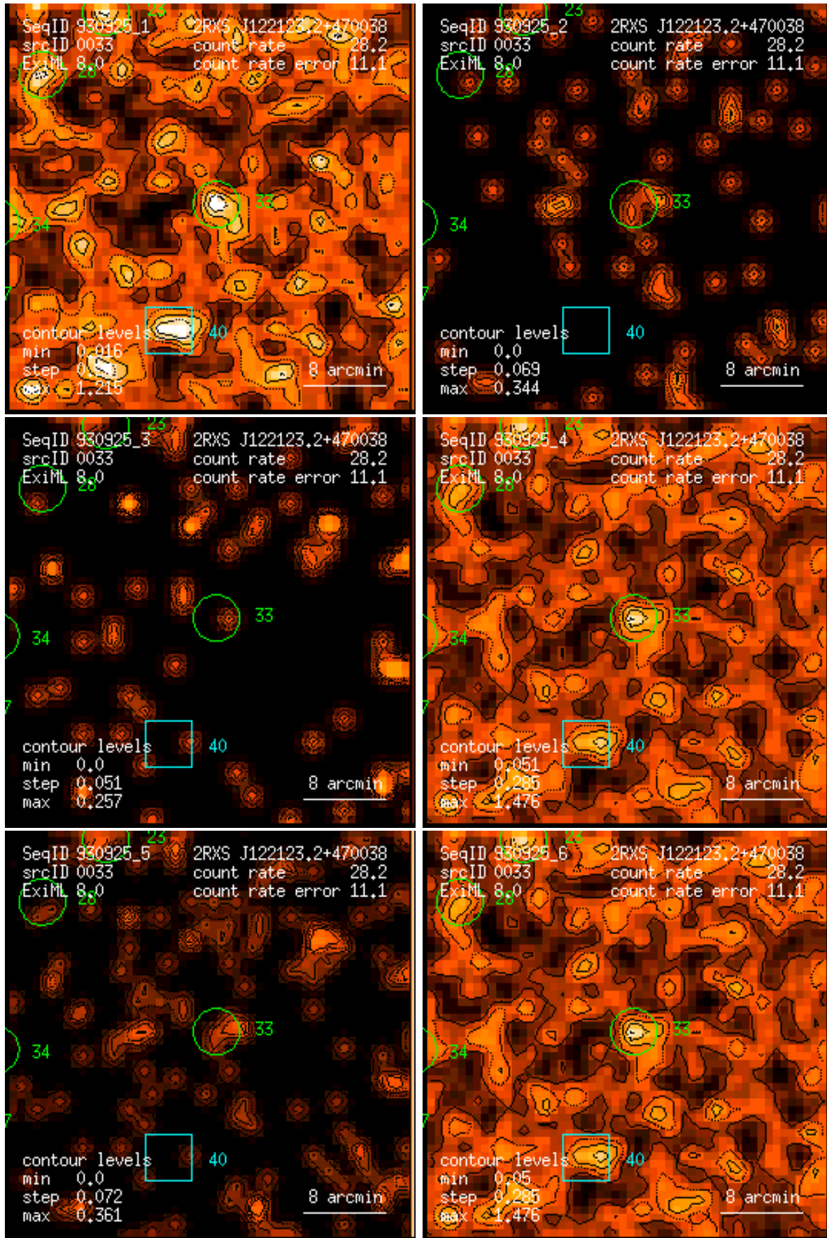
Figure 33: RASS 930925: detection 0033: band rate images, Gaussian filter: (1) PSPC channels 11 – 41, (2) 52 – 90, (3) 91 – 201, (4) 11 – 235, (5) 52 – 201, (6) 11 – 201. Broad band rates in counts/ks. Band rate contour levels in counts/ks/arcmin 2 .
