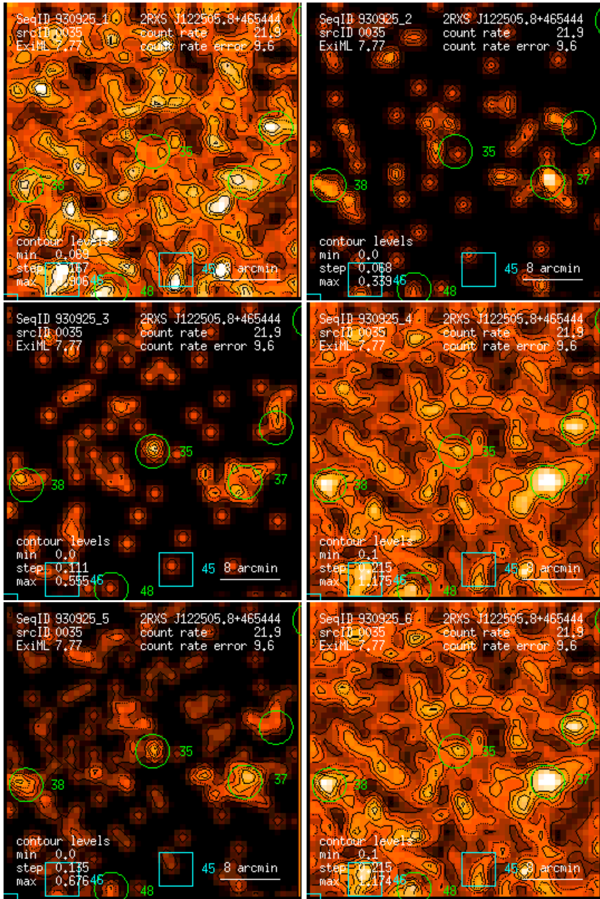
Figure 35: RASS 930925: detection 0035: band rate images, Gaussian filter: (1) PSPC channels 11 – 41, (2) 52 – 90, (3) 91 – 201, (4) 11 – 235, (5) 52 – 201, (6) 11 – 201. Broad band rates in counts/ks. Band rate contour levels in counts/ks/arcmin 2 .
