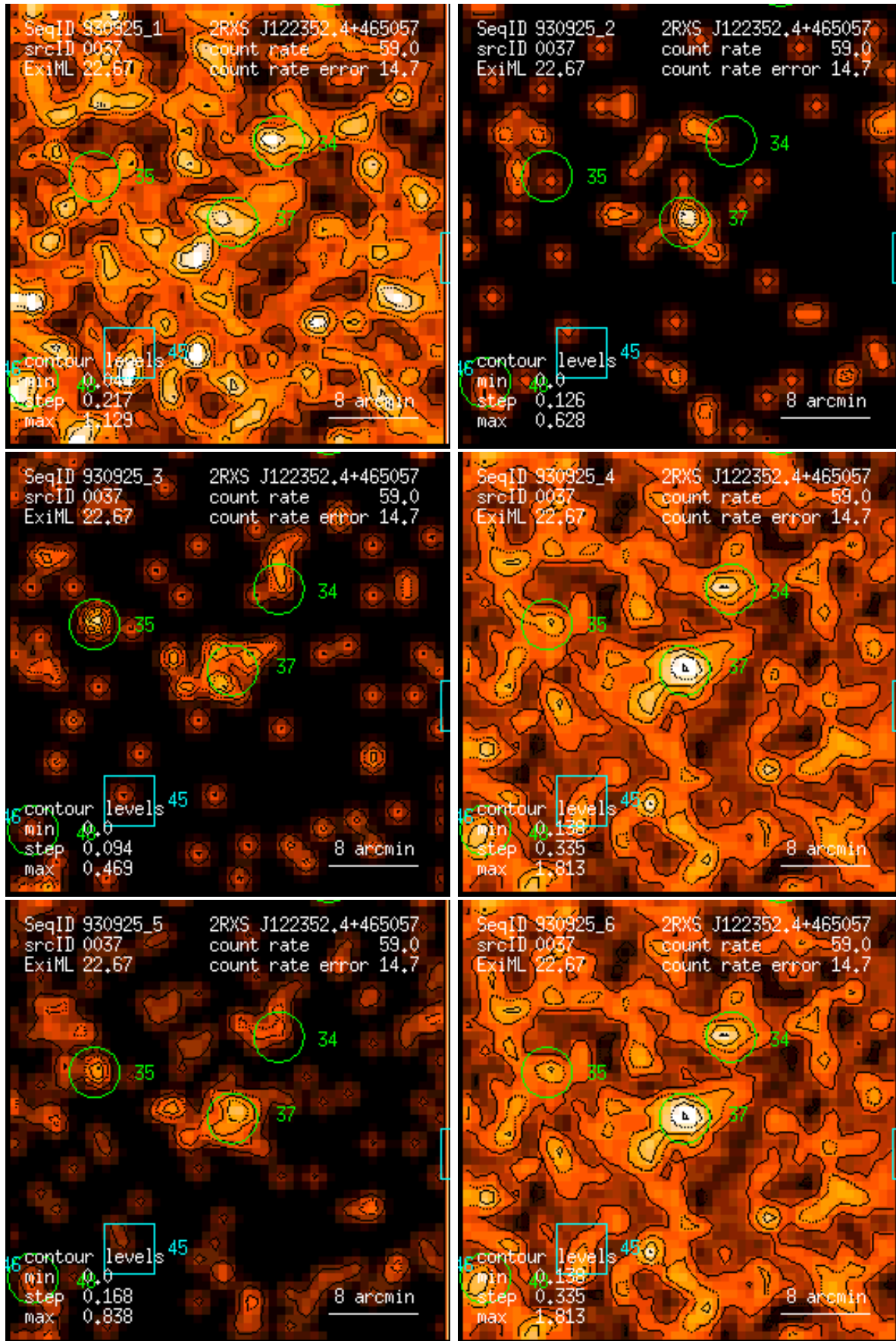
Figure 37: RASS 930925: detection 0037: band rate images, Gaussian filter: (1) PSPC channels 11 – 41, (2) 52 – 90, (3) 91 – 201, (4) 11 – 235, (5) 52 – 201, (6) 11 – 201. Broad band rates in counts/ks. Band rate contour levels in counts/ks/arcmin 2 .
