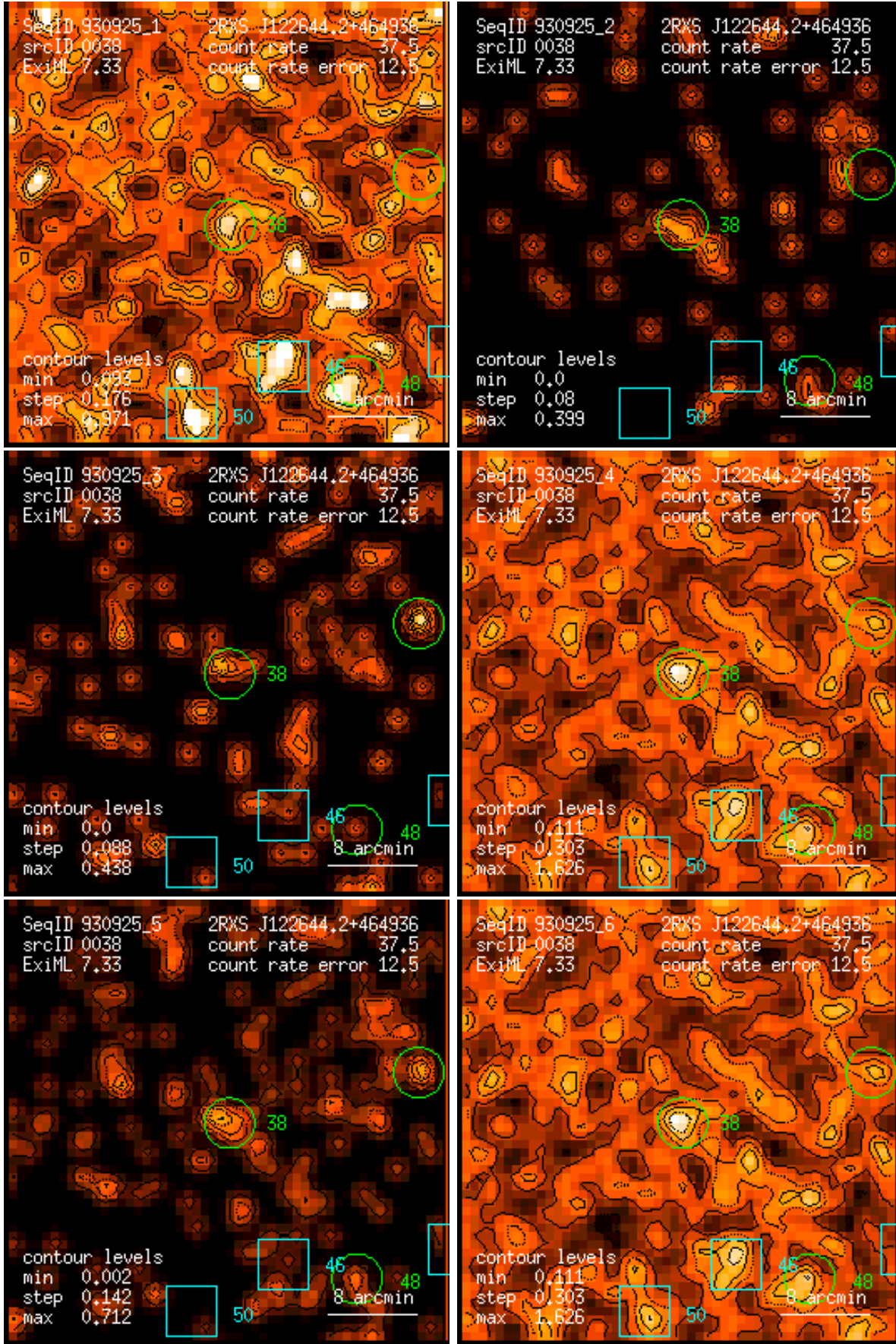
Figure 38: RASS 930925: detection 0038: band rate images, Gaussian filter: (1) PSPC channels 11 – 41, (2) 52 – 90, (3) 91 – 201, (4) 11 – 235, (5) 52 – 201, (6) 11 – 201. Broad band rates in counts/ks. Band rate contour levels in counts/ks/arcmin 2 .
