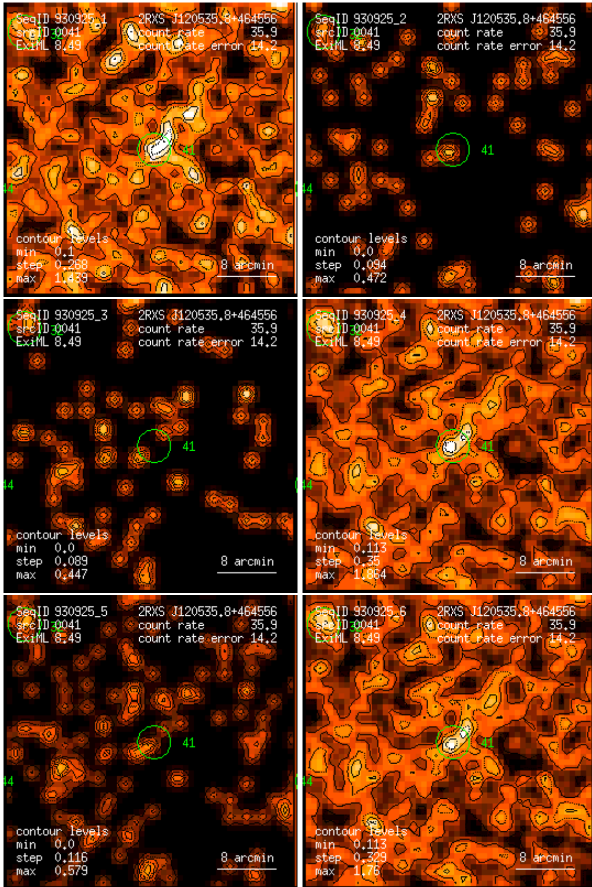
Figure 41: RASS 930925: detection 0041: band rate images, Gaussian filter: (1) PSPC channels 11 – 41, (2) 52 – 90, (3) 91 – 201, (4) 11 – 235, (5) 52 – 201, (6) 11 – 201. Broad band rates in counts/ks. Band rate contour levels in counts/ks/arcmin 2 .
