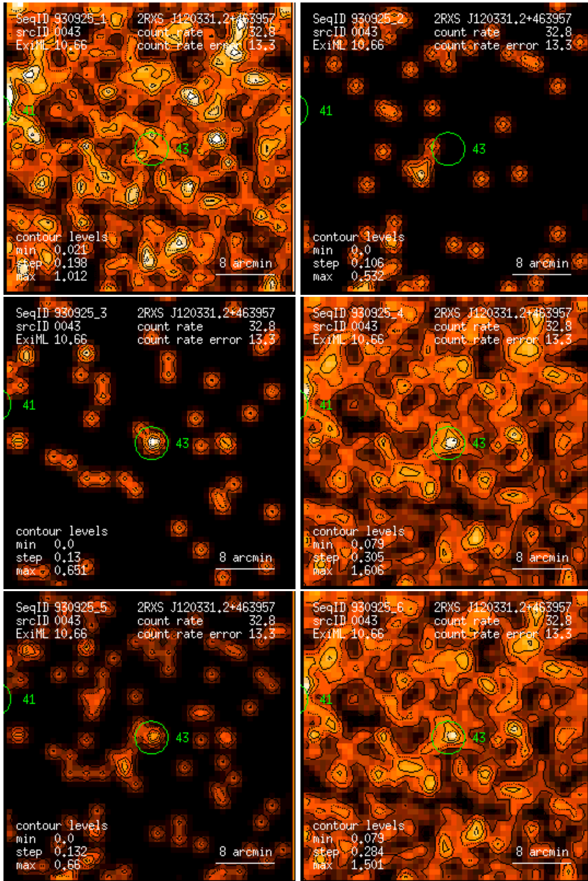
Figure 43: RASS 930925: detection 0043: band rate images, Gaussian filter: (1) PSPC channels 11 – 41, (2) 52 – 90, (3) 91 – 201, (4) 11 – 235, (5) 52 – 201, (6) 11 – 201. Broad band rates in counts/ks. Band rate contour levels in counts/ks/arcmin 2 .
