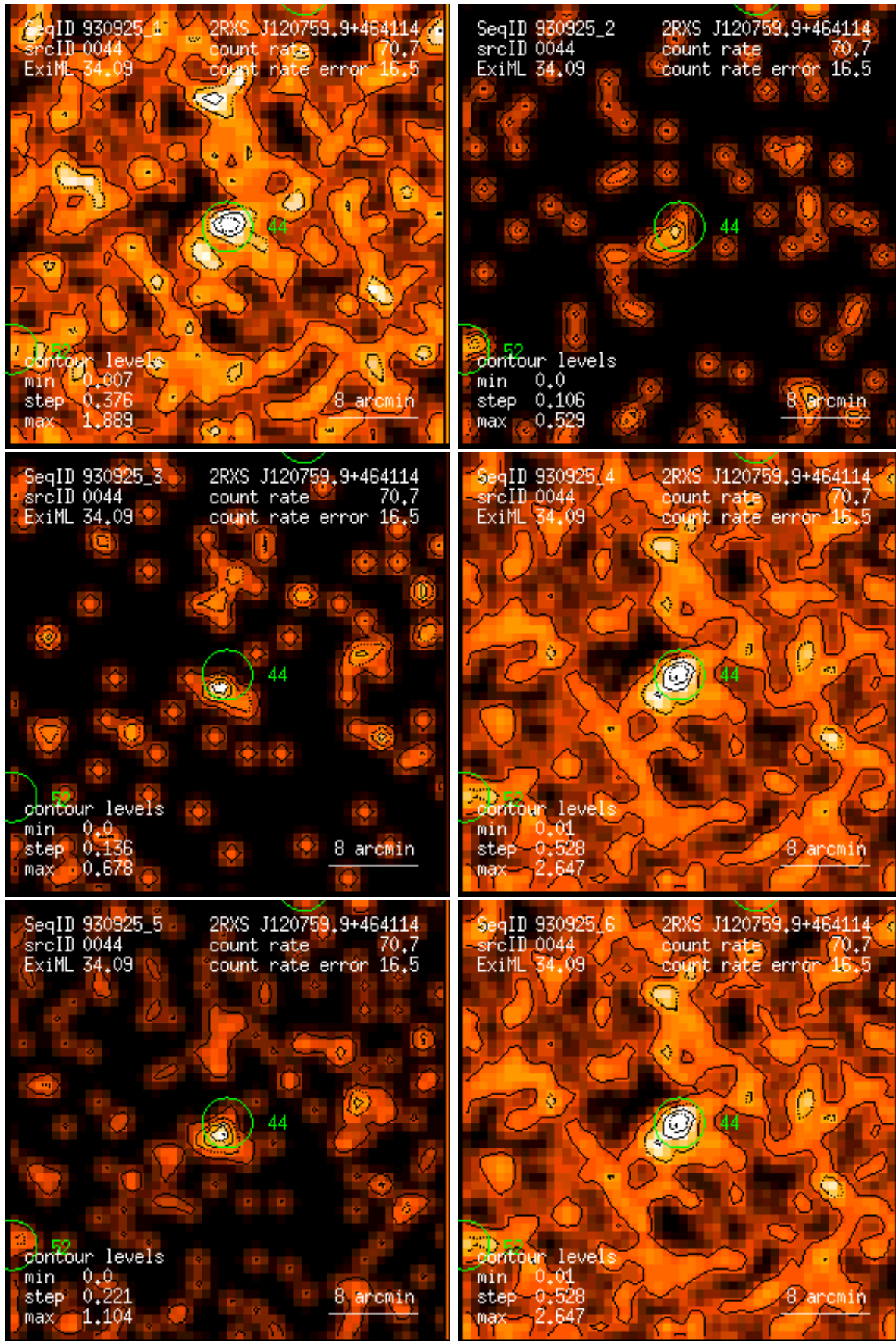
Figure 44: RASS 930925: detection 0044: band rate images, Gaussian filter: (1) PSPC channels 11 – 41, (2) 52 – 90, (3) 91 – 201, (4) 11 – 235, (5) 52 – 201, (6) 11 – 201. Broad band rates in counts/ks. Band rate contour levels in counts/ks/arcmin 2 .
