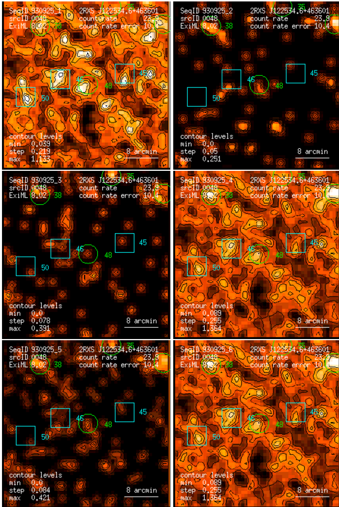
Figure 48: RASS 930925: detection 0048: band rate images, Gaussian filter: (1) PSPC channels 11 – 41, (2) 52 – 90, (3) 91 – 201, (4) 11 – 235, (5) 52 – 201, (6) 11 – 201. Broad band rates in counts/ks. Band rate contour levels in counts/ks/arcmin 2 .
