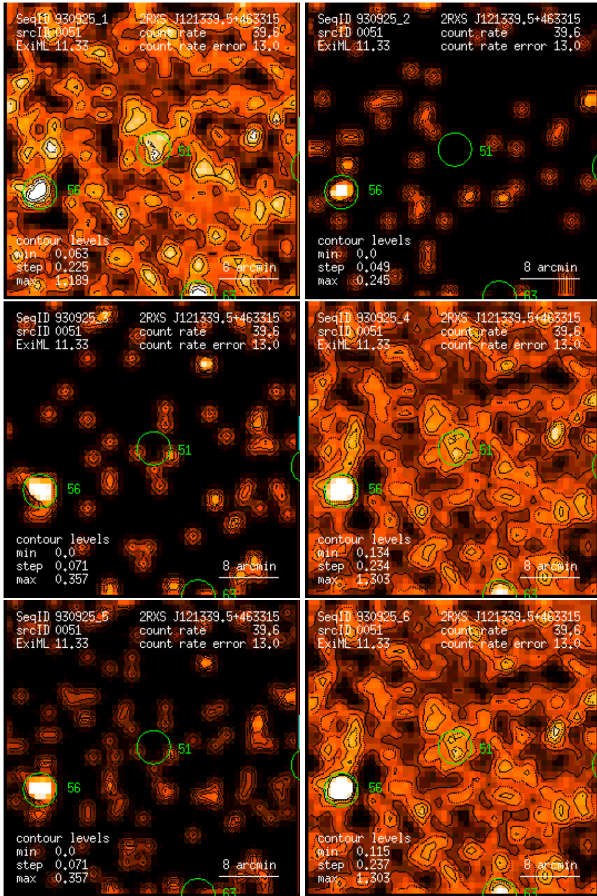
Figure 51: RASS 930925: detection 0051: band rate images, Gaussian filter: (1) PSPC channels 11 – 41, (2) 52 – 90, (3) 91 – 201, (4) 11 – 235, (5) 52 – 201, (6) 11 – 201. Broad band rates in counts/ks. Band rate contour levels in counts/ks/arcmin 2 .
