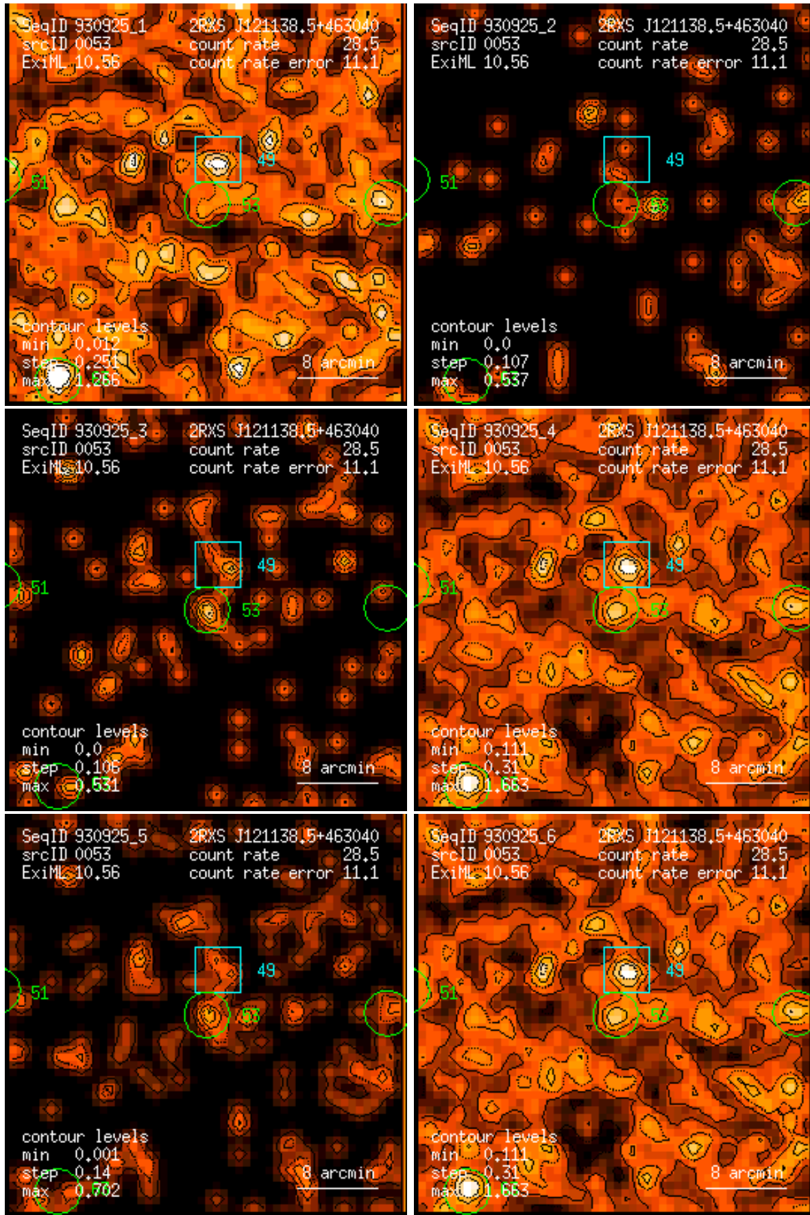
Figure 53: RASS 930925: detection 0053: band rate images, Gaussian filter: (1) PSPC channels 11 – 41, (2) 52 – 90, (3) 91 – 201, (4) 11 – 235, (5) 52 – 201, (6) 11 – 201. Broad band rates in counts/ks. Band rate contour levels in counts/ks/arcmin 2 .
